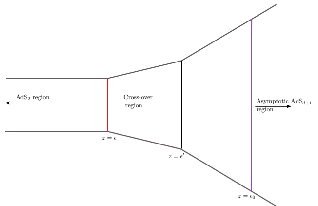
FIG. 2: A simple sketch of extremal black hole geometries with an infinite AdS 2 throat and the process of defining effective field theories via the holographic Wilsonian RG flow. To extract low energy physics, it is convenient to integrate out the bulk geometry all the way to the boundary of AdS 2 , i.e. z = \epsilon surface in the figure. The induced effective action on z = \epsilon can be interpreted as multiple-trace deformations of the CFT 1 dual to AdS 2 .
