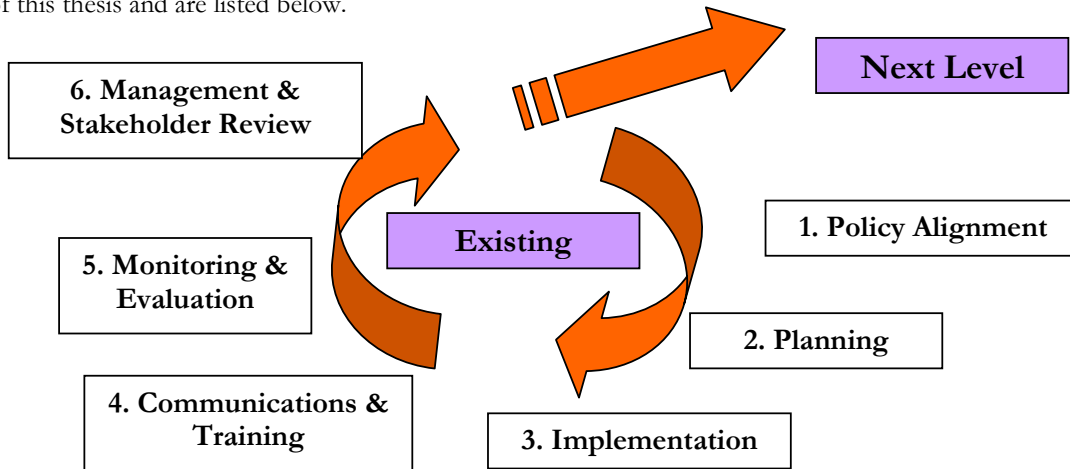
Figure 12: SEMS Framework
