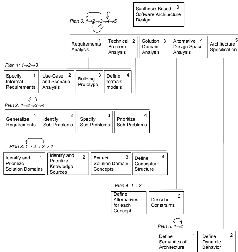
Fig. 3. Synthesis-based Software Architecture Design
