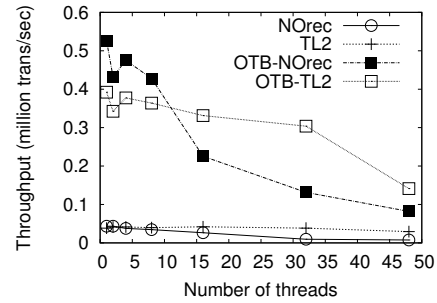
(a) linked-list
