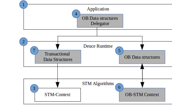
Figure 1. New design of DEUCE framework.
