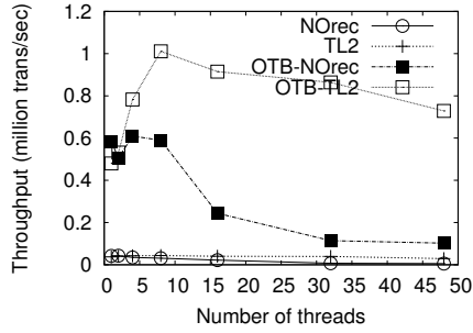
(a) 80% add/remove, 20% contains
