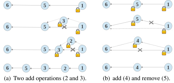
Figure 2. Executing more than one operation that involves the same node in the same transaction.
