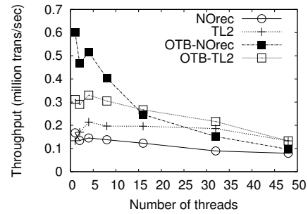
(b) skip-list
