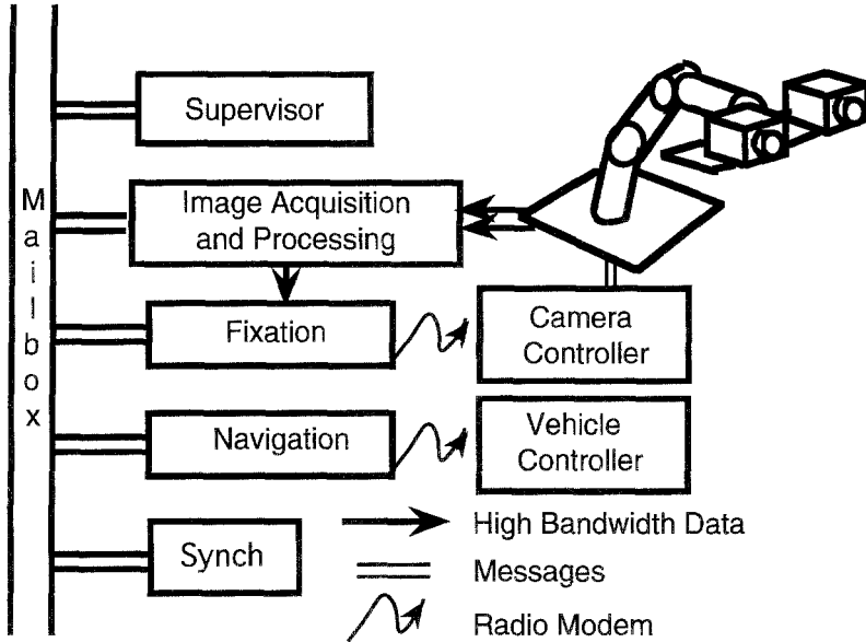
Figure 3 Configuration of demonstration system within the SAVA III Vision test-bed.
