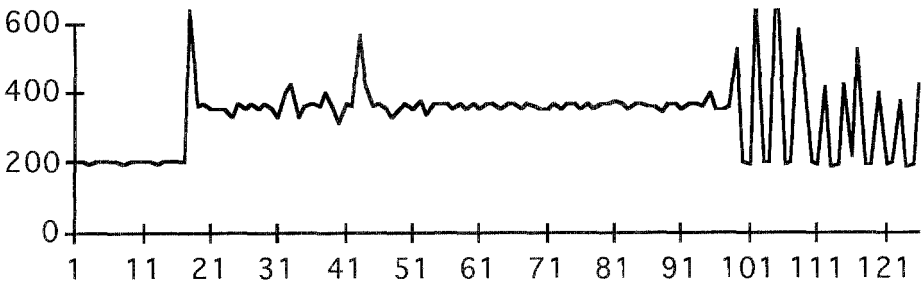
Figure 4. Timing diagram for image acquisition and processing from a typical tracking session. Vertical axis is milliseconds. The horizontal axis is the cycle number.
