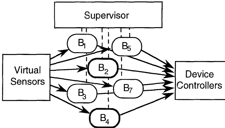
Figure 1 . A Supervisory controller selects and controls the sequencing of perceptual processes. Multiple processes can be active at the same time. Arrows indicate flow of data, dashed lines indicate control, the highlighted ellipses are currently active.
