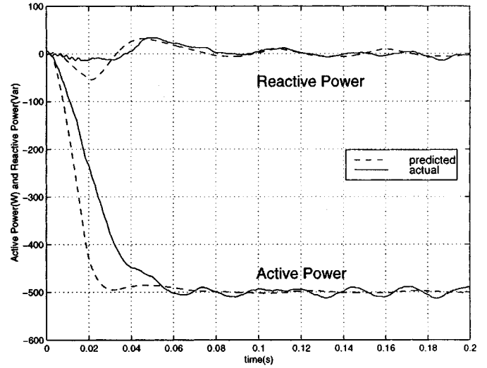
Fig. 7. Step change in active power.
