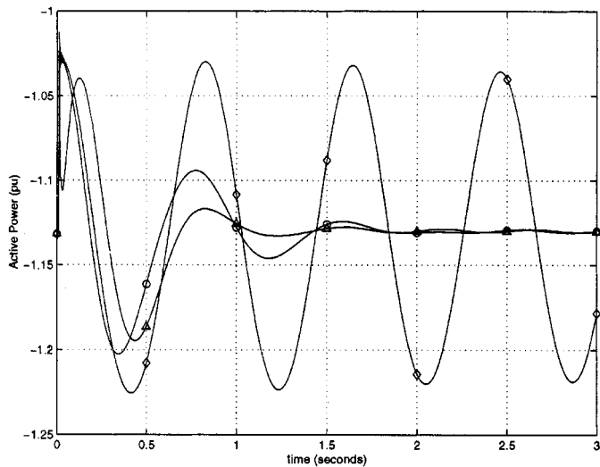
Fig. 12. Active power flow between areas ( \diamond —no control, \circ —StatCom, \triangle —StatCom/BESS).
