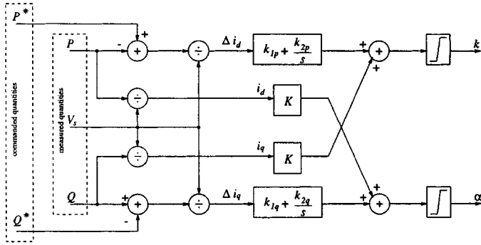
Fig. 5. Decoupled PQ control.
