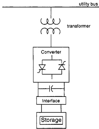
Fig. 1. Integrated StatCom with energy storage.
