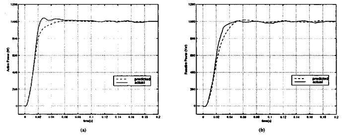
Fig. 8. Simultaneous step change of active and reactive power from 0 to 1 kW and 1 kVar (respectively).
