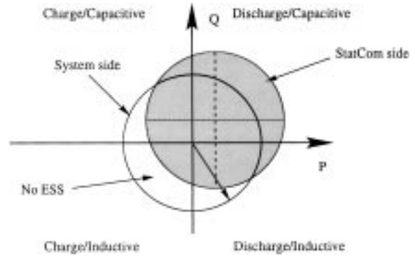
Fig. 3. StatCom/BESS output power characteristics.
