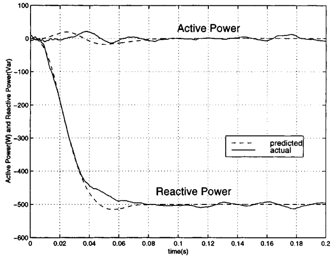
Fig. 6. Step change in reactive power.
