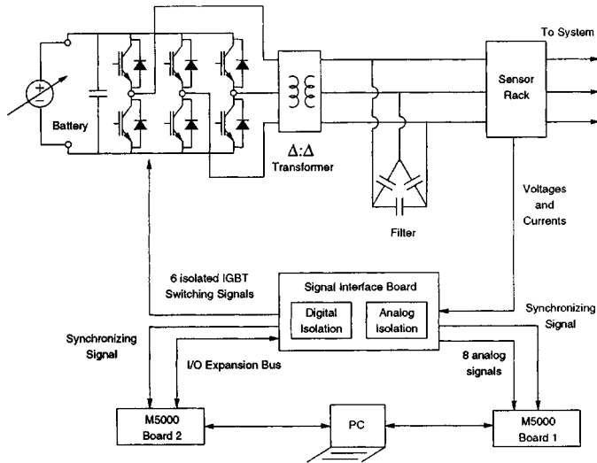
Fig. 4. Experimental StatCom/BESS.
