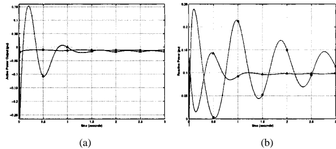
Fig. 13. (a) Active power outlet. (b) Reactive power output ( \circ —StatCom, \triangle —StatCom/BESS).
