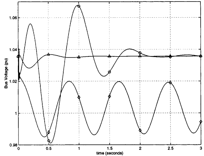
Fig. 11. Voltage at Bus 6 ( \diamond —no control, \circ —StatCom, \triangle —StatCom/BESS).
