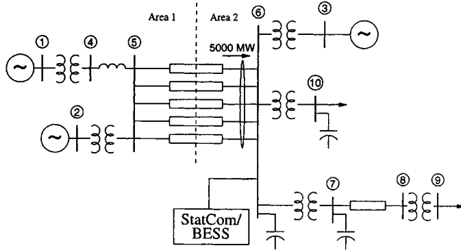
Fig. 10. Example system for comparison of controls.
