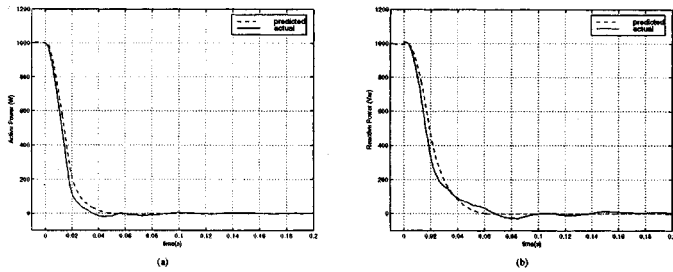
Fig. 9. Simultaneous step change of active and reactive power to 0.
