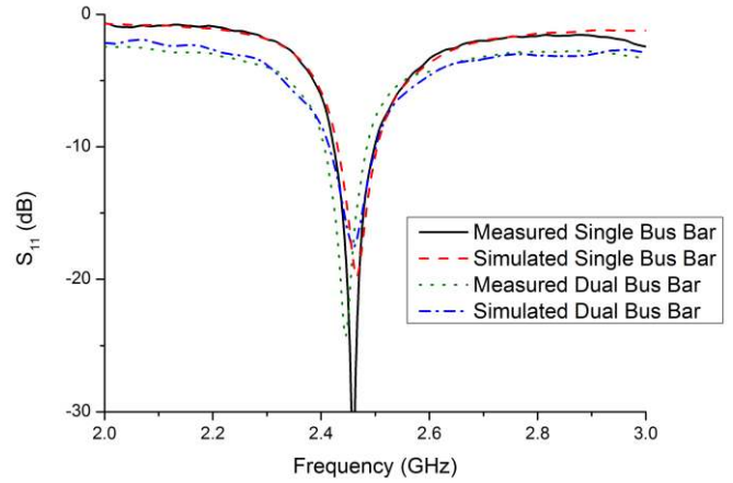
Fig. 3. Measured and simulated antenna S_{11} results
