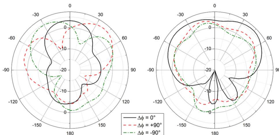
Fig. 7. Measured beam switching for array phase offset ( \Delta\phi ) in X-Z plane (left) and Y-Z plane (right)
