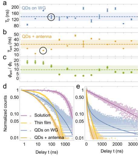
Figure 4: PL lifetime from different freestanding pillars of PbS/CdS QDs (a) and PbS/CdS QDs placed in the gap of plasmonic bowtie antennas (b) extracted from measurements with different SNSPDs. The quantum efficiency with an antenna \phi_{ant} normalized to an isolated pillar \phi_0 in (c) correspond to the lifetime measurements above. The dashed lines and shaded areas show the respective mean value and standard deviation, the displayed error bars are the 1-\sigma confidence intervals from the fit. The PL decay traces in (d) and (e) were normalized after subtraction of the background, the experimental data is overlaid with fitted stretched exponential functions. The circled data points in (a) and (b) were extracted from the respective decay traces in (d) and (e).
