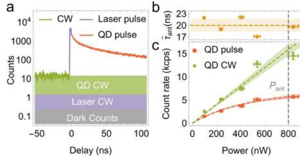
Figure 3: (a) PL decay trace recorded for QDs placed in the antenna gap using an excitation power of P_{ant} = 800 nW. (b) Excitation power dependence of the mean lifetime extracted from a stretched exponential fit. (c) Power dependence of the pulsed and CW contribution of the QD emission. The shaded areas show the 1- \sigma confidence intervals from the fit displayed as a dashed line.
