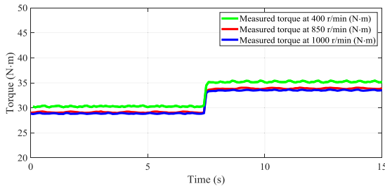
FIGURE 18. Measured torque at 400 r/min, measured torque at 850 r/min and measured torque at 1000 r/min when torque reference steps from 30 N·m to 35 N·m.
