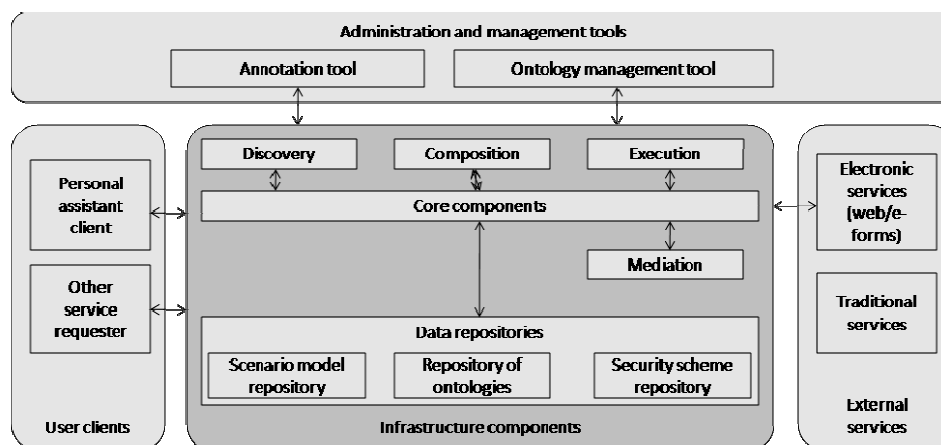
Figure 3: Access-eGov architecture
