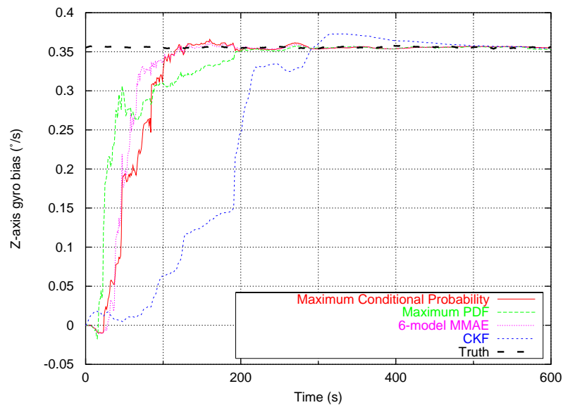
Figure 7.19: MPDF and MCP filter z -axis gyro bias alignment
