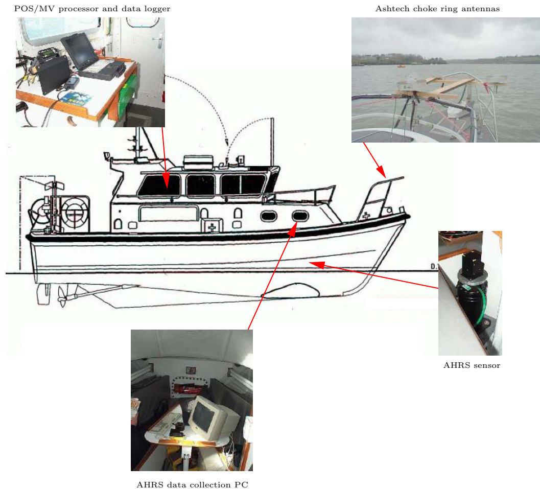
Figure 8.1: Marine trial sensor configuration
