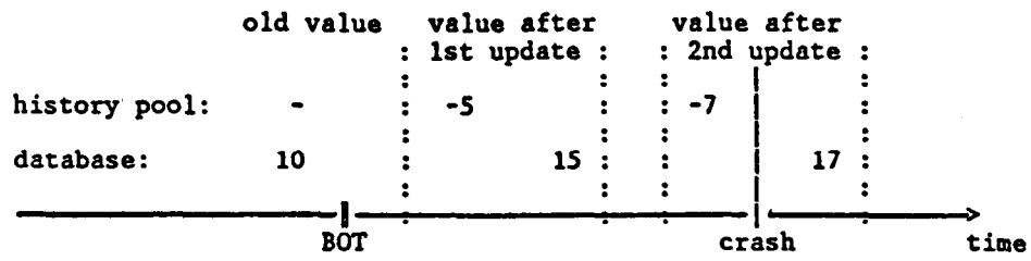
FIGURE 5: Delta Creation in the Case of Repeated Updates
