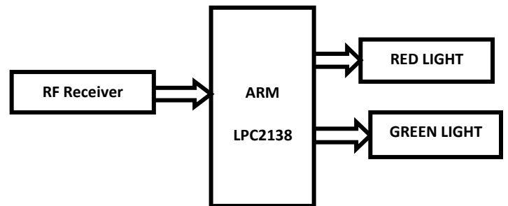
Fig5: block diagram of traffic junction unit
