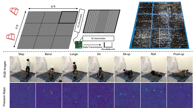
Figure 2. Tactile data acquisition hardware. Top: Our recording set-up includes a tactile sensing carpet spanning 36 \text{ ft}^2 with 9,216 sensors (upper right), the corresponding readout circuits, and 2 cameras. Bottom: Typical pressure maps captured by the carpet from diverse human poses and activities.
