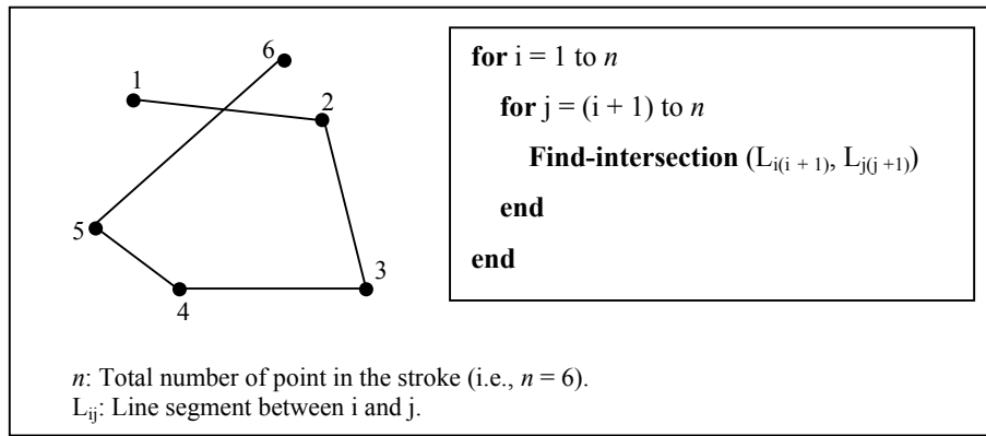
Figure 3. General algorithm to find intersection point
