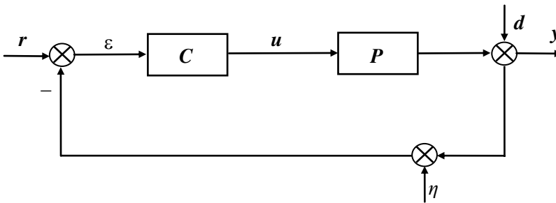
Fig. 6 – Basic configuration of a stabilization system
