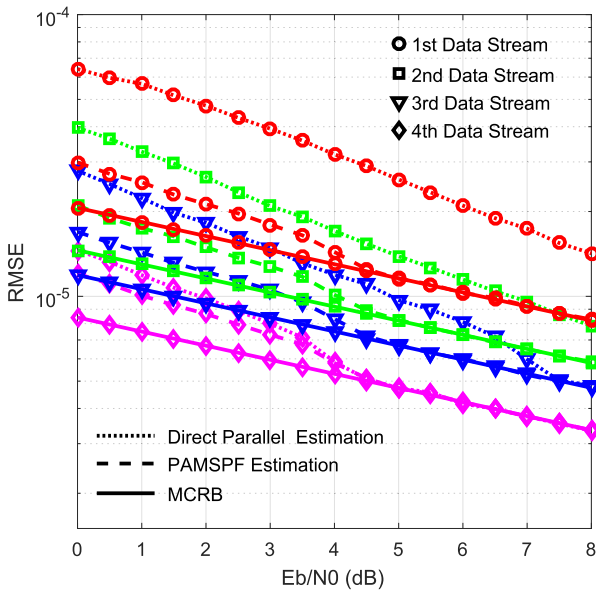
FIGURE 12. RMSE of the frequency and phase offset estimation in MCICSC system, where the polar code of C_1(2048, 1024) is employed: (a). RMSE of frequency offset estimation for C_1 while specifying \Delta fTs = 5.0 \times 10^{-5} in MCICSC system; (b). RMSE of phase offset estimation for C_1 while specifying \theta = 0.2\pi in MCICSC system.
