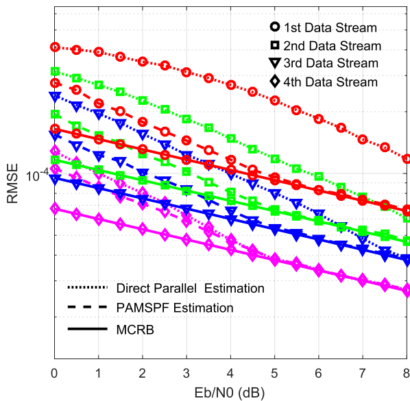
FIGURE 14. RMSE of the frequency and phase offset estimation in MCICSC system, where the polar code of C_3(512, 256) is employed: (a). RMSE of frequency offset estimation for C_3 while having \Delta fTs = 2.0 \times 10^{-4} in MCICSC system; (b). RMSE of phase offset estimation for C_3 while specifying \theta = 0.2\pi in MCICSC system.
