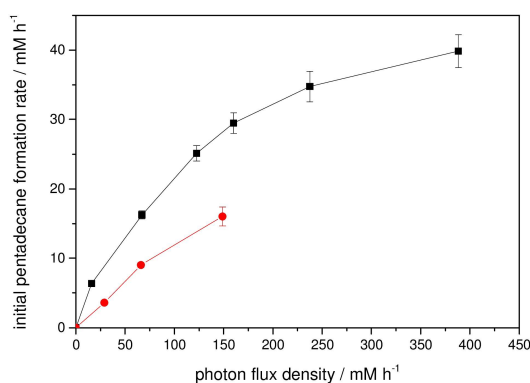
Figure 4. Comparison of the initial pentadecane formation rate using WLEs for internal illumination (■) and a LED for external illumination (●) at different light intensities. Conditions: [palmitic acid] 0 = 13 mM; [rec. E. coli ] = 50 g L -1 ([CvFAP] = 6 μM); buffer: 100 mM Tris-HCl (pH 8.5), 30% v/v DMSO, volume = 50 mL; T = 20 °C. The variation of the internal illumination light intensity was achieved by addition of different numbers of WLEs while for external illumination this was realized by changing the driver current.
