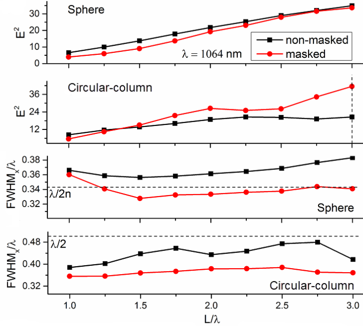
Figure 2 Statistics of maximum E^2 field intensities and FWHM/ \lambda for the models of the spherical and circular-column particle-lenses ranged from L/\lambda = 1 to 3 with and without the mask apodization.
