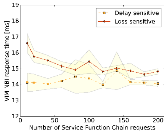
FIGURE 7 Average NBI response time and 95% confidence interval at the SDN/cloud VIM with increasing number of service chain requests.
