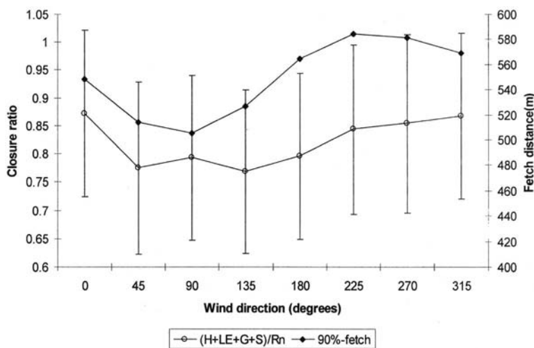
Fig. 2. Energy balance closure ratio ( H + \lambda E + G + S/R_n ) and fetch distance plotted against wind direction bin-averaged for each 45° for the 1999 growing season. Error bars are one standard deviation.
