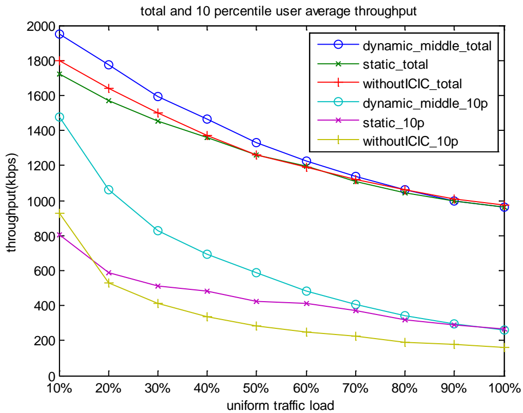
Figure17.Total and 10 percentile user average throughput with uniform traffic load in cross building employed intermediate level dynamic scheme
