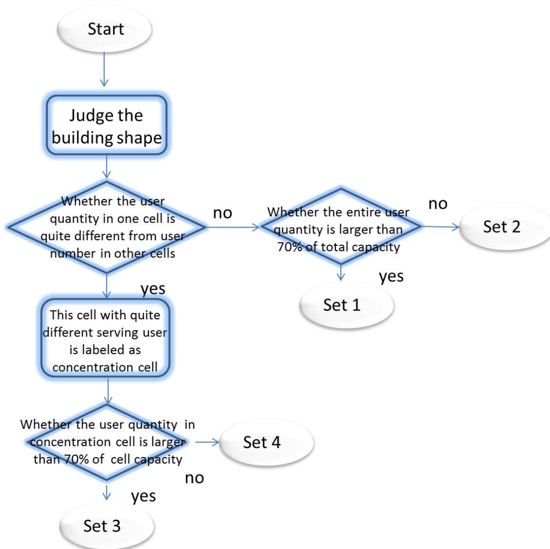
Figure8. Diagram of low level dynamic scheme for symmetric building cell
