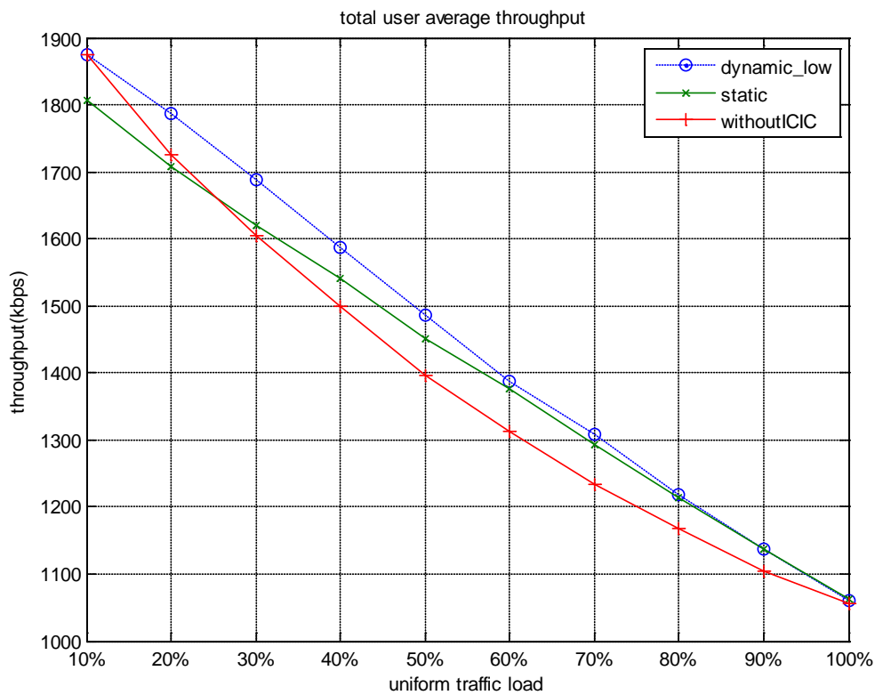
Figure15.Total user average throughput with uniform traffic load in concentric square building
