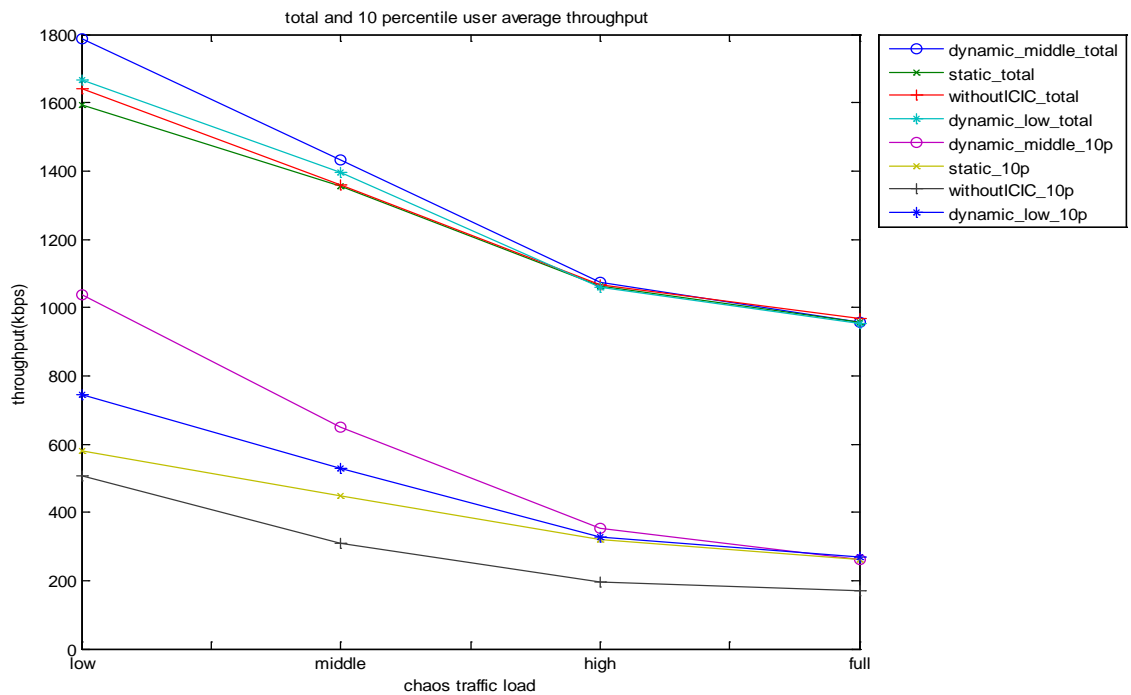
Figure20. User average throughput with chaos traffic load in cross building
