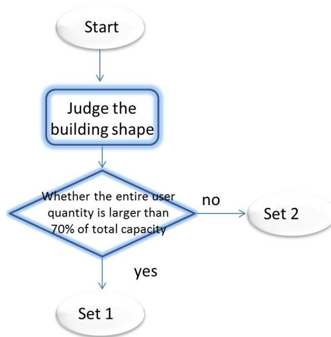
Figure7. Diagram of low level dynamic scheme only based on total user number
