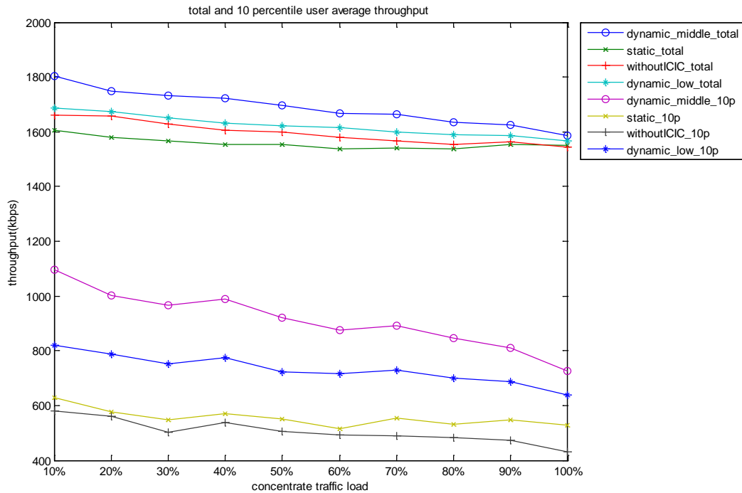
Figure18. User average throughput in cross building with concentration traffic load at wing position
