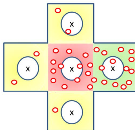
Figure11(b). Best frequency allocation with heterogeneous traffic load
