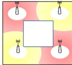
Figure12(b).frequency scheduling with 2 sub-bands in square building
