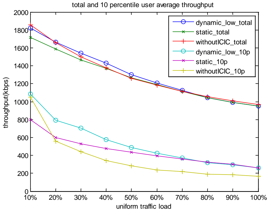
Figure 16. Total and 10 percentile user average throughput with uniform traffic load in cross building
