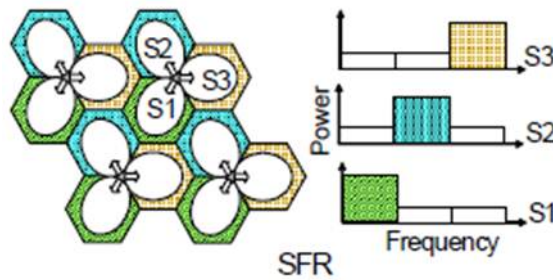
Figure4. Soft frequency reuse scheme [14]
