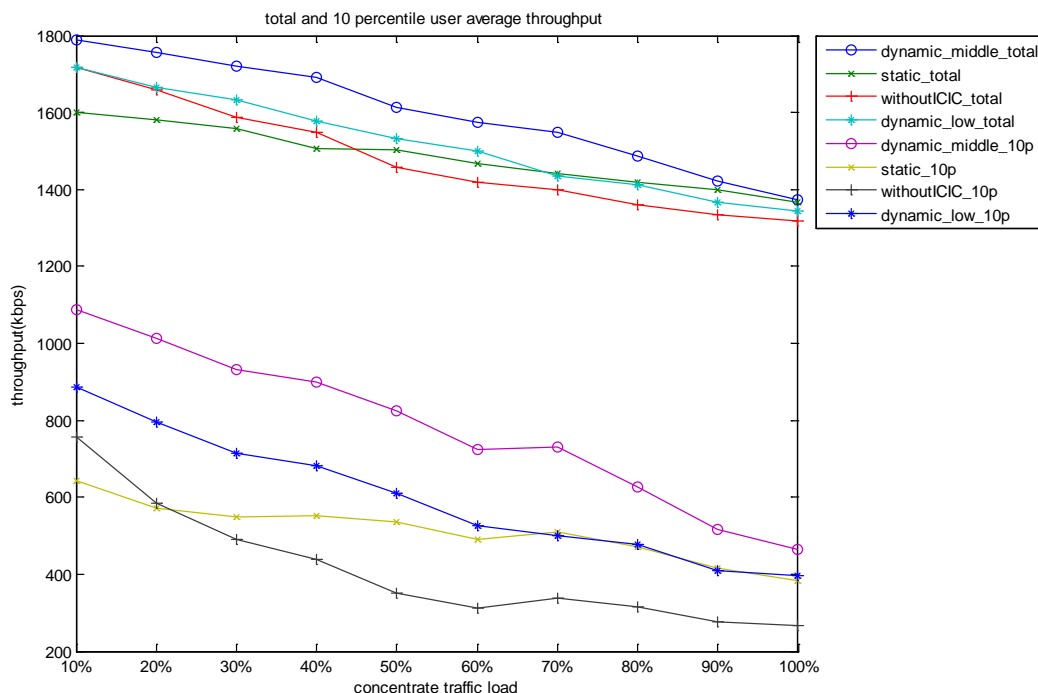
Figure19. User average throughput in cross building with concentration traffic load in central location
