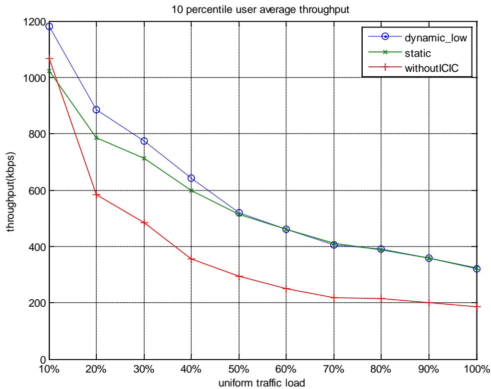
Figure14. 10 percentile user average throughput with uniform traffic load in concentric square building
