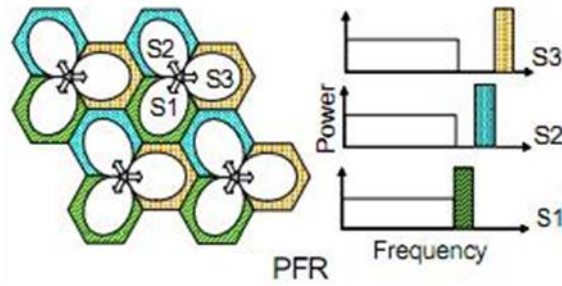
Figure3. Partial frequency reuse scheme [14]
