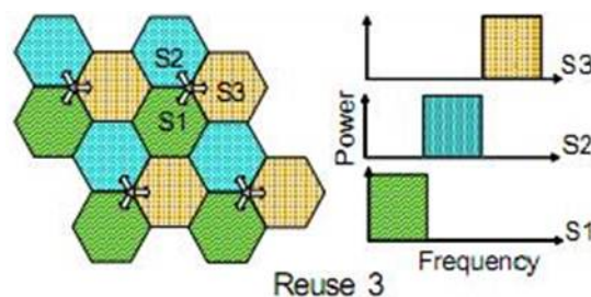
Figure2. Hard frequency reuse scheme with reuse 3 [14]
