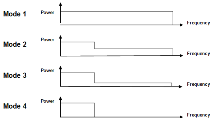
Figure6. Adaptive FFR modes[15]
