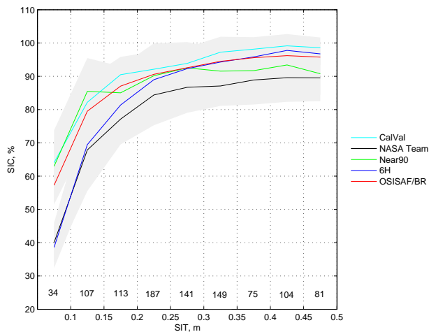
Figure 4. Sea ice concentration (SIC) calculated by the SIC algorithms (shown in colours) as a function of SMOS sea ice thickness (SIT) in areas of the Arctic Ocean, which are known to be \sim 100\% thin ice during the time period from 1 October to 12 December 2010. Grey shading shows standard deviations of the algorithms. Number of measurements in each bin is shown above the x axis (total number is 991). In this SIC range OSISAF is the same as BR.
