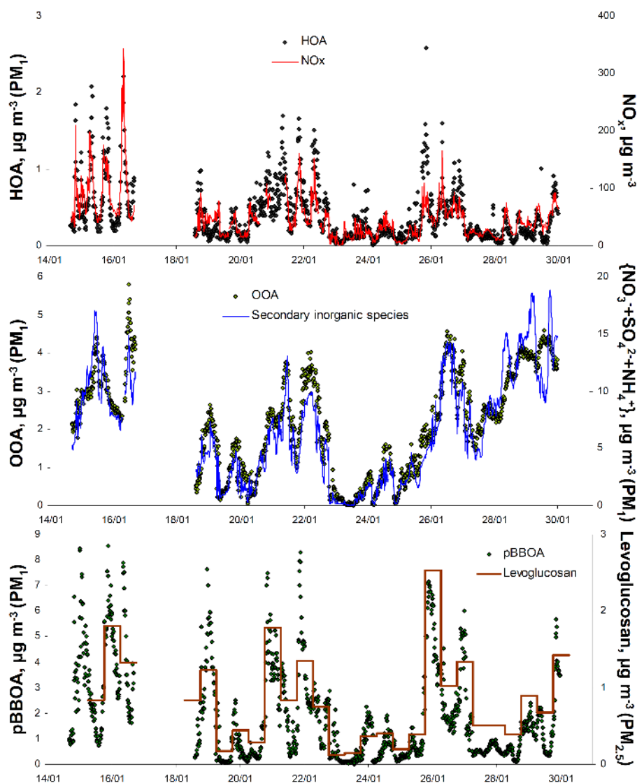
Fig. 6. Time series of each PMF factor (3-factorial PMF, “FPEAK” = −0.2 and “seed” = 0) along with some of their corresponding tracers (NO x , secondary inorganic species and levoglucosan respectively for HOA, OOA and pBBOA).
