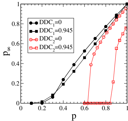
Fig. 3: (Colour on-line) Simulation results for ER networks each of size N=100000 and \langle k \rangle=3.75 showing the effect of changing the degree-degree correlation (DDC) within a single network (solid symbols) compared to the effect in two interdependent networks (open symbols). For the case of interdependent networks the DDC is measured within each network and the IDDC and ICC are kept zero. Even though the effect of the DDC on a single network is minor (solid circles) it significantly decreases the robustness of interdependent networks (open circles).
