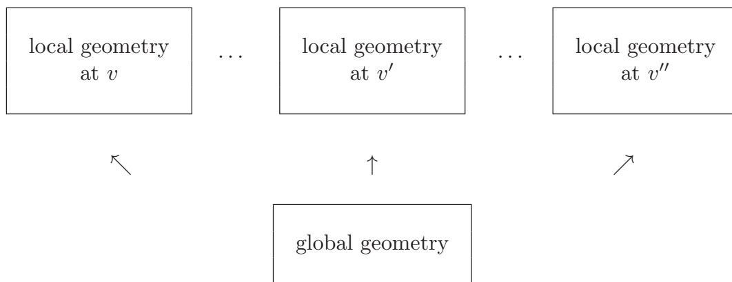
Fig. 4.3: Globalizability
