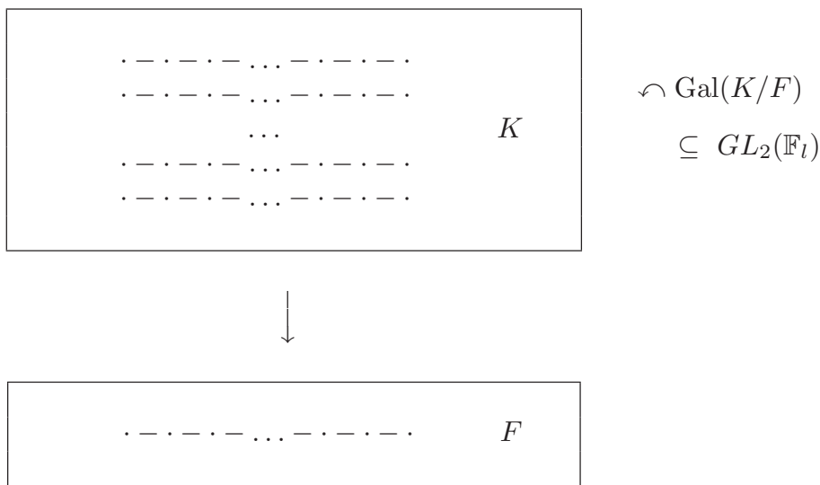
Fig. 4.1: Prime-strips as “sections” of \text{Spec}(K) \rightarrow \text{Spec}(F)
