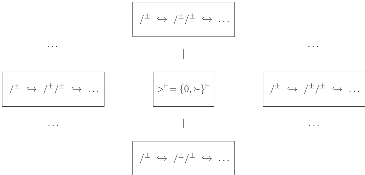
Fig. 6.3: Étale-picture of \mathcal{D}-\Theta^{\pm\text{ell}} -Hodge theaters
