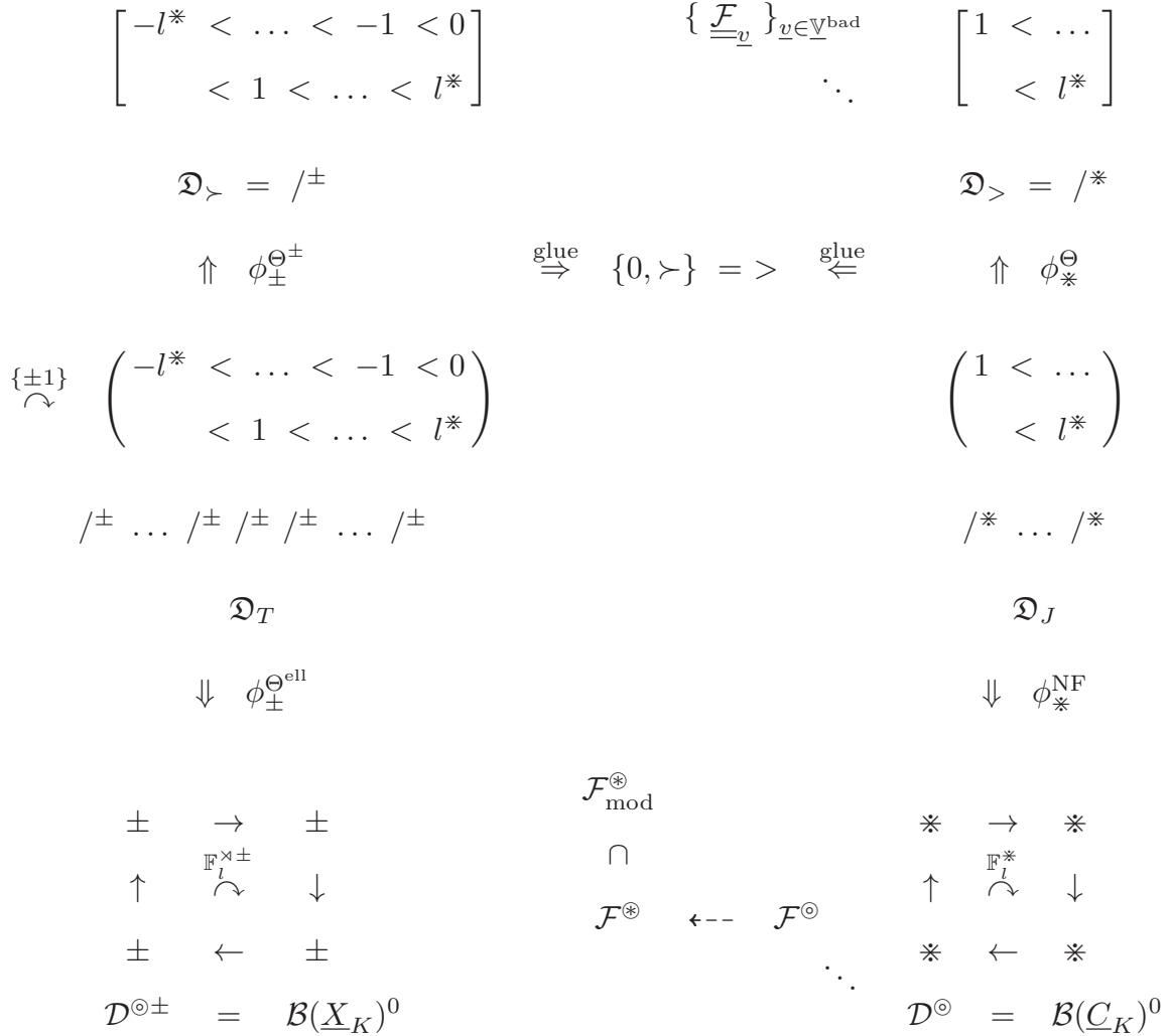
Fig. 6.5: The combinatorial structure of a \Theta^{\pm \text{ell}} NF-Hodge theater [cf. also Figs. 4.4, 4.7, 6.1, 6.3, 6.6]
