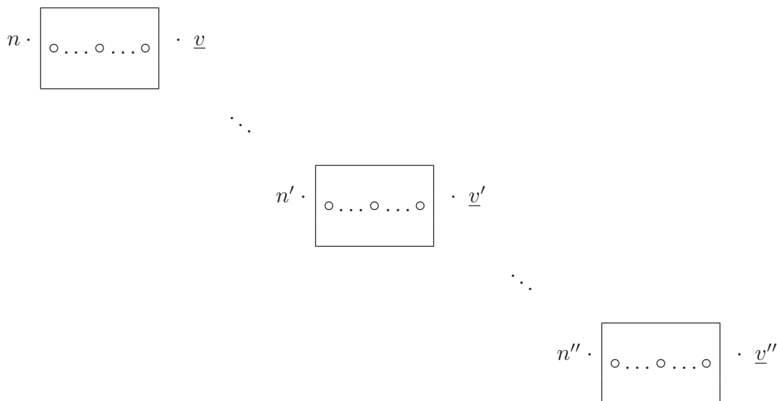
Fig. 5.1: Constant distribution
