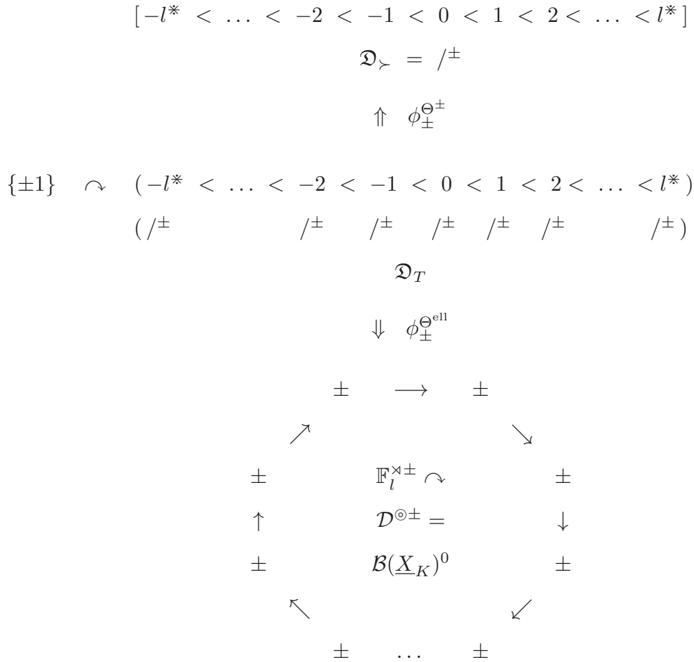
Fig. 6.1: The combinatorial structure of a \mathcal{D}\text{-}\Theta^{\pm\text{ell}} -Hodge theater
