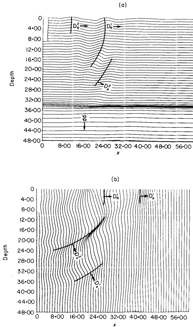
Figure 6. Section of a half plane with a slot to the right of the axis of symmetry at time level t\alpha/h = 60 . The displacements are amplified by the factors; (a) 4, (b) 8. D_p^i , D_s^i , D_i^i ; i = 1, 2 are the diffracted compressional, shear and Rayleigh pulses respectively. D/L = 1/2 , l/D = 4/9 .
