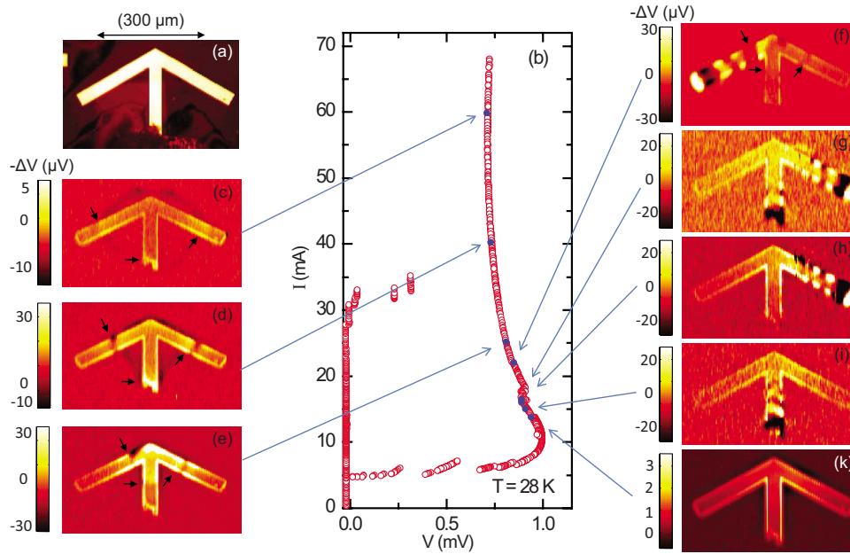
FIG. 9. (Color online) (a) Optical image, (b) current voltage characteristic, and [(c)–(k)] LTSLM images of the arrow-shaped sample 1, as measured at T=28 K. [(c)–(f)] Black arrows in images indicate edge of hot spot.
