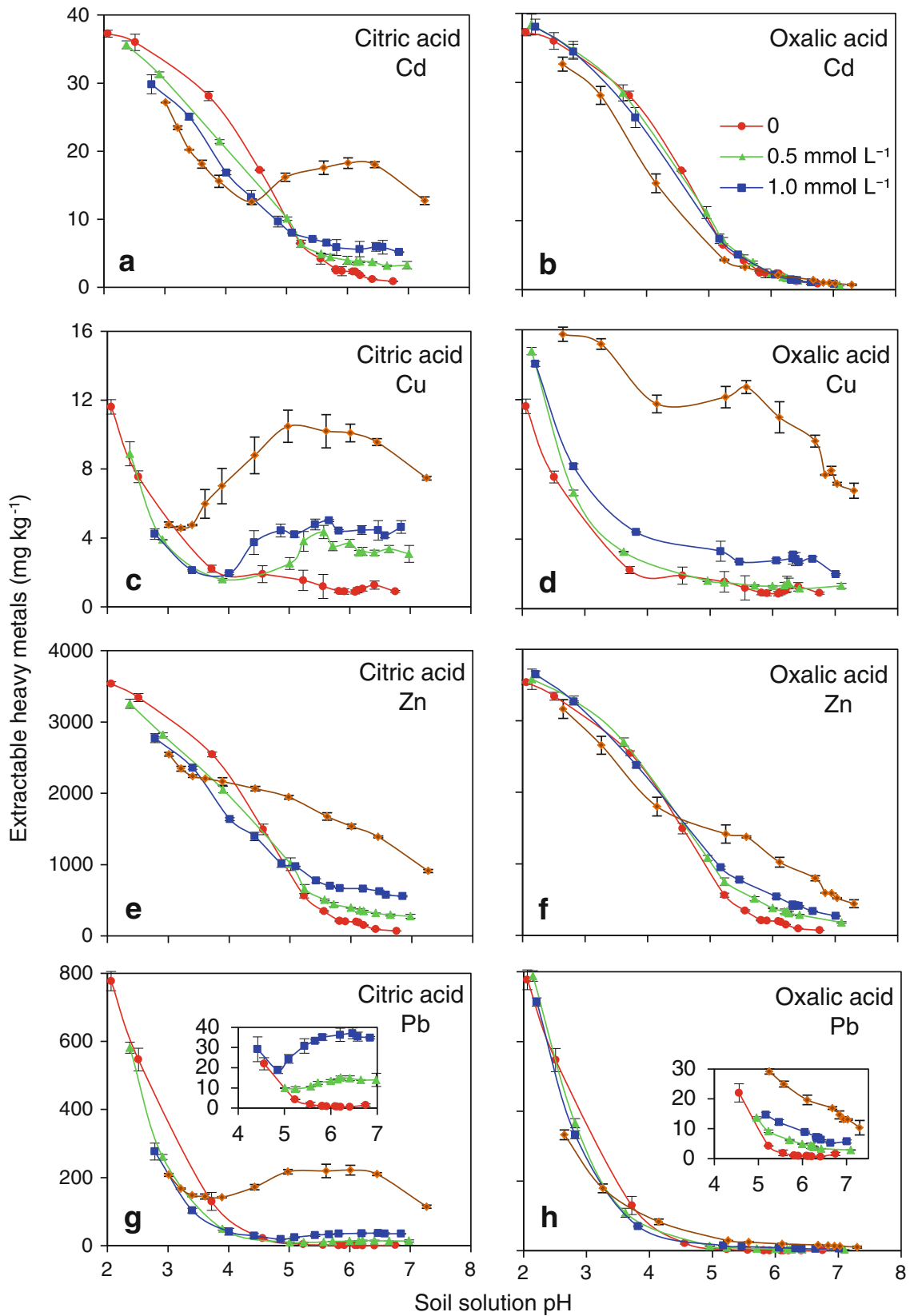
Fig. 2 Extraction of Pb, Cd, Zn and Cu from Daxin soil by citric acid and oxalic acid as a function of pH. Error bars represent standard deviations of triplicate measurements
