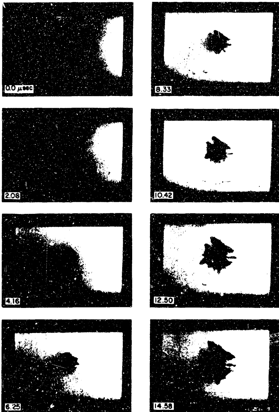
FIG. 17 HEAD-ON VIEW OF 0.458 CALIBER AP BULLET — GLASS BLOCK IMPACT AT 1800 ft sec (2.08 \mu\text{sec} between frames)
