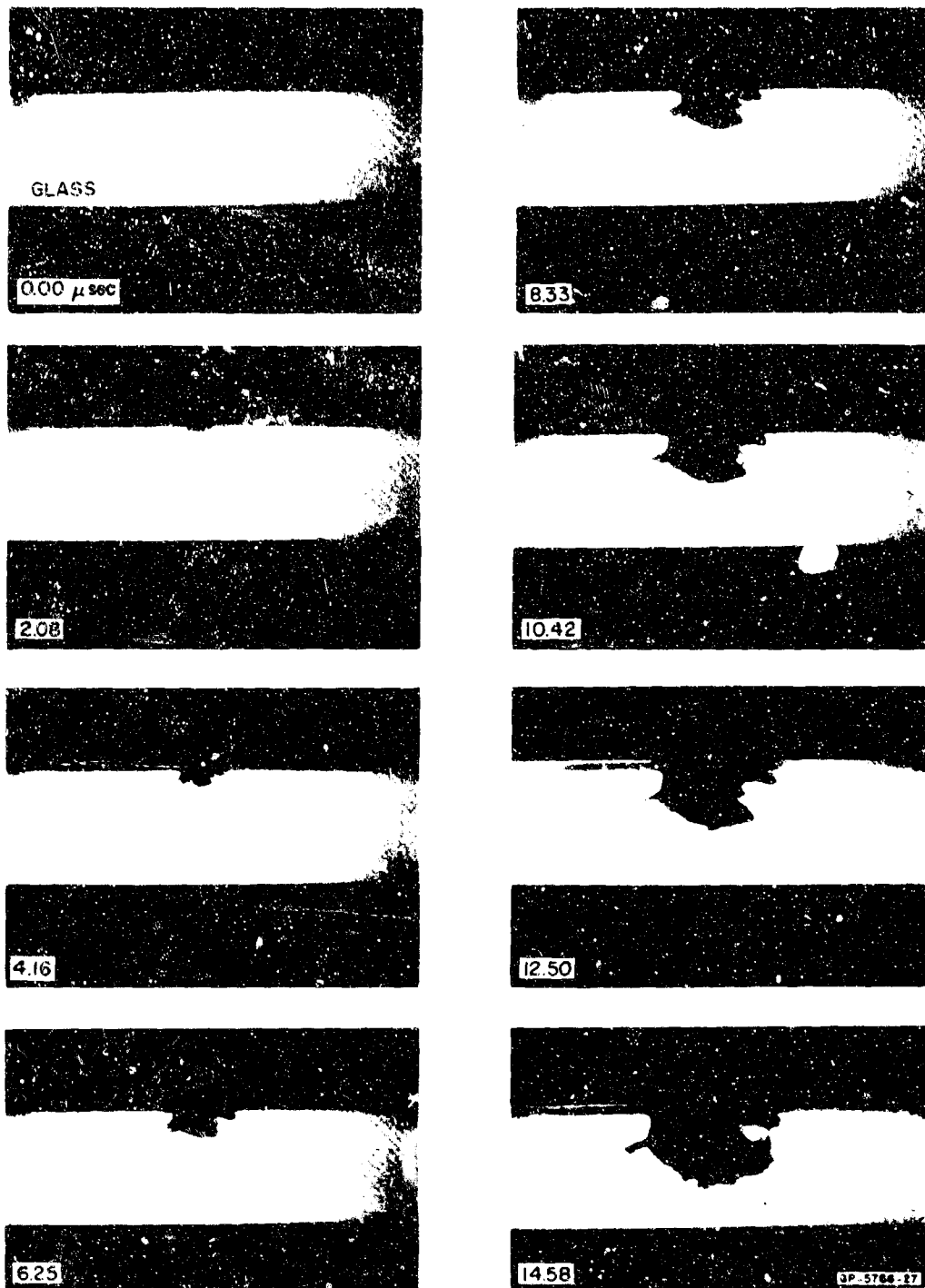
FIG. 15 INTERNAL PROFILE VIEW OF 0.458 CALIBER AP BULLET — GLASS BLOCK IMPACT AT 1800 ft/sec (2.08 \mu sec between frames)
