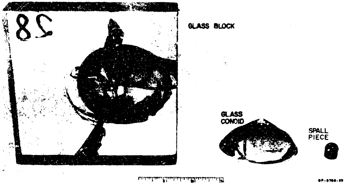
FIG. 32 GLASS BLOCK AFTER IMPACT AT 94 ft/sec WITH A 0.5-INCH-DIAMETER SPALL PIECE
