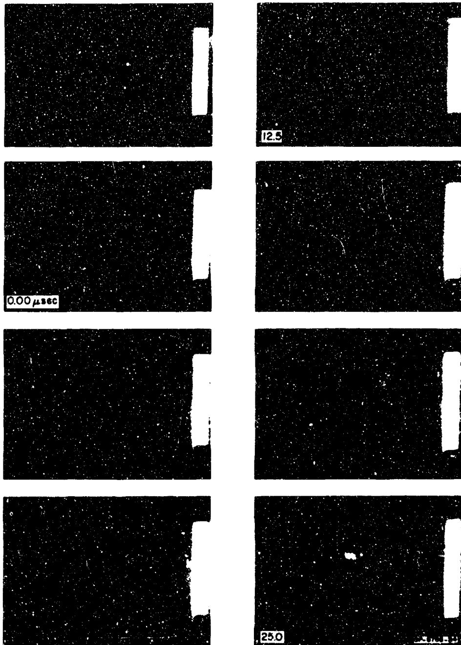
FIG. 9 OBLIQUE REAR VIEW OF 0.458 CALIBER AP BULLET — CERAMIC TILE IMPACT AT 1800 ft/sec (4.17 μsec between frames)
