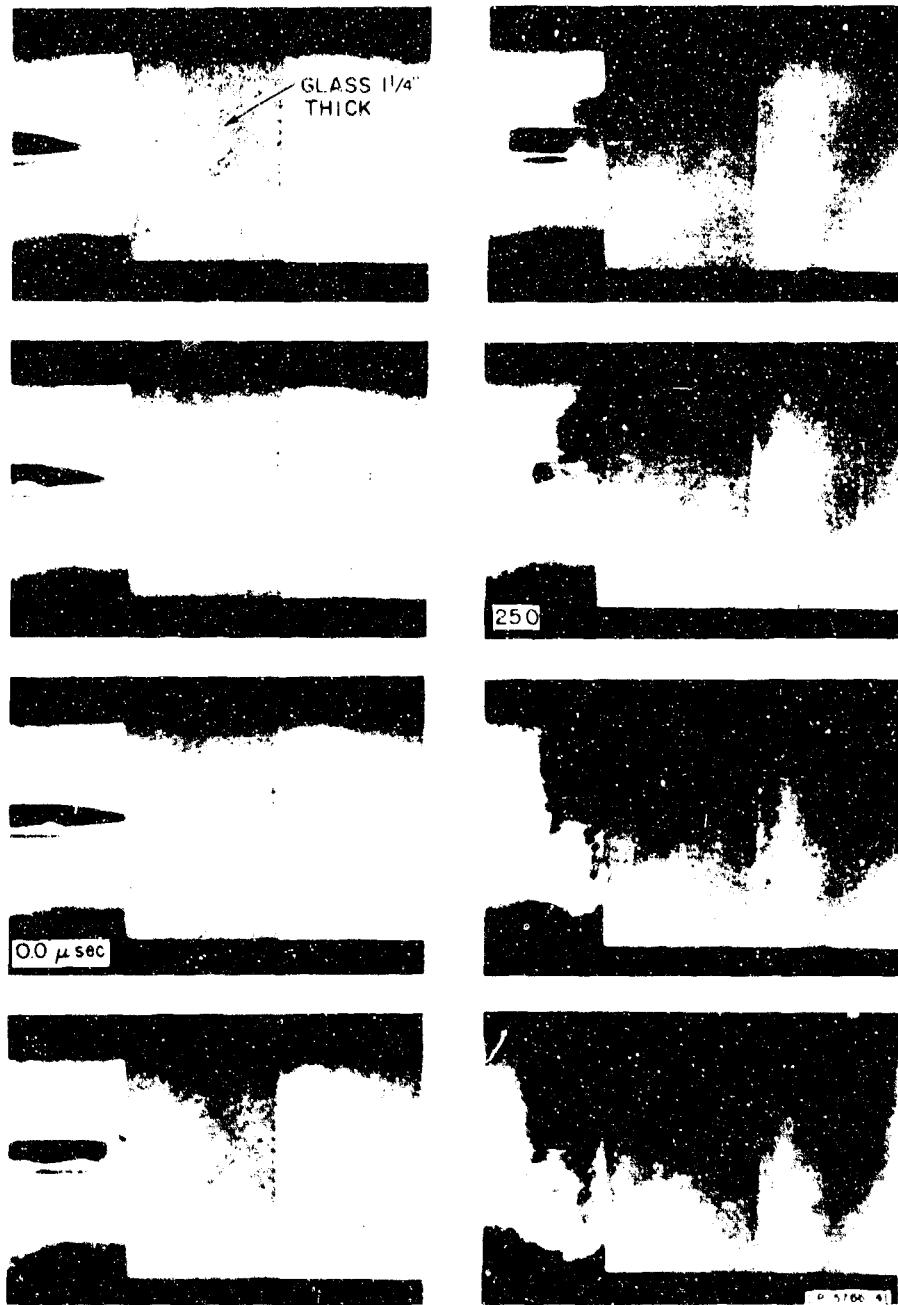
FIG. 30 EXTERNAL VIEW OF 0.3 CALIBER STANDARD AP BULLET — GLASS BLOCK IMPACT AT 2400 ft./sec (8.33 \mu sec between frames)
