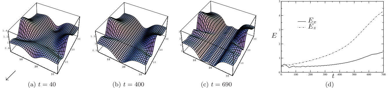
FIG. 3: Same as for Fig. 2 with for \delta = 1.33 , \eta = 0.05 , \mathcal{M} = 0.674 , B = 1.82 and \text{Pr} = 7 . The Reynolds number is \text{Re} = 2 .
