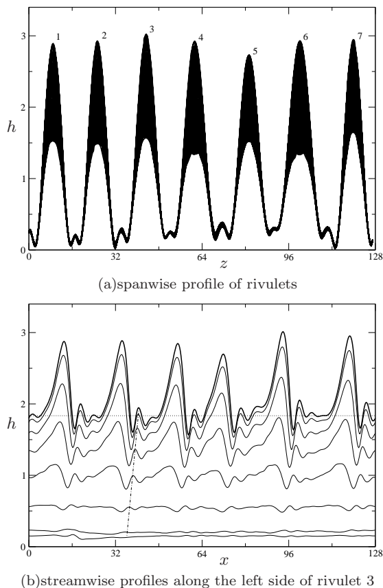
FIG. 8: Cross-sections of Fig. 5a for Re = 2 : (a) 128 profiles are drawn, hence the dark area. (b) the dashed line shows the approximative local substrate thickness of the profile at the crest (thick solid line). The dot-dashed line is the locus of a local maximum, which shows the curvature of the wave front.
