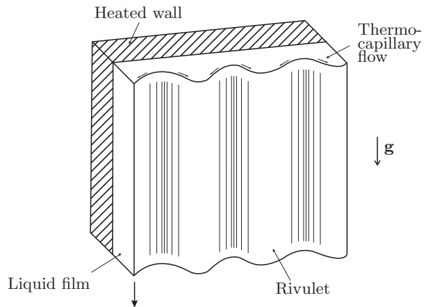
FIG. 1: Rivulet structure driven by thermocapillary effect at the surface of a falling liquid film heated from the wall.
