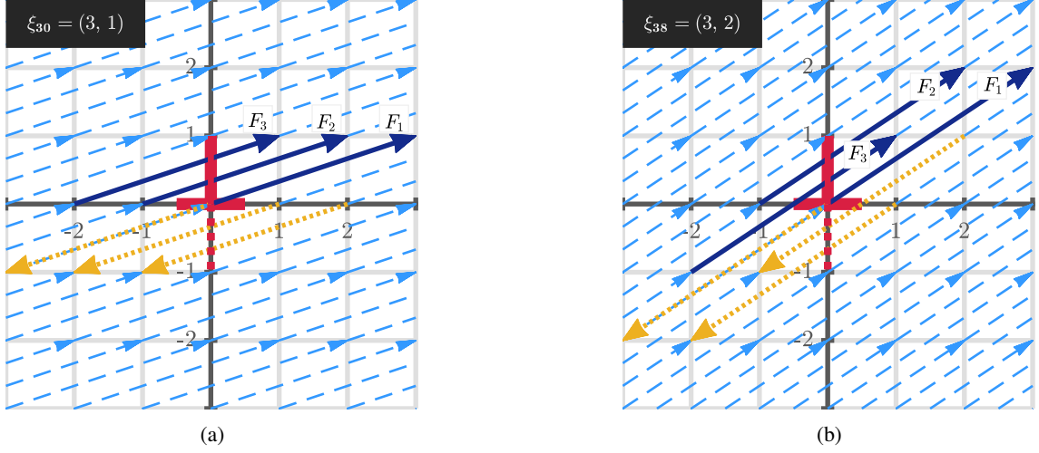
FIG. 3: Illustration of the force vectors along the vectors \xi_\alpha (of the Q49ZOTT lattice in Fig. 1) that belong to symmetry group \hat{z} and pass through (bold solid arrows) the vertical infinitesimal d\mathbf{A}^{(y)} unit area element (red bold solid line). The unlabeled bold dotted arrows which pass through the red bold dotted line ( d\mathbf{A}^{(y)} ) are accounted for along \xi_\alpha . In both cases, it is clear that considering contributions to d\mathbf{A}^{(y)} correctly accounts for those passing through the horizontal infinitesimal d\mathbf{A}^{(x)} unit area element (red bold solid line) centered at \mathbf{x} . (a) For vector \xi_{30} there are six ( 2\mathcal{E}^z ) force vectors with equal contribution to \mathcal{P}_{ij}^{int, \hat{z}=10} . (b) For vector \xi_{38} there are also six force vectors, however, they do not contribute equally to \mathcal{P}_{ij}^{int, \hat{z}=13} . The contributions to \hat{z} = 10 are automatically considered in Eq. (16), whereas those in \hat{z} = 13 can still be obtained with Eq. (16) but require a unique condition ( C_\beta ) to correct the different contributions of \mathbf{F}_2 and \mathbf{F}_3 (see the text).
