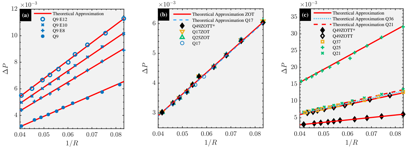
FIG. 8: (Color online) Laplace experiment for the single static circular droplet test including intra- and inter-interactions for 11 different lattice models. The numerical results (symbols) are obtained by setting the initial R_o [in Eq. (D2)] and then at equilibrium, by postprocessing, measuring the actual R and calculating the difference between the equation of state, computed by Eqs. (9) and (17), of the two bulk phases, i.e., \Delta P = P_o^\phi - P_o^\varphi . The theoretical approximations (lines) are obtained by computing \sigma from Eqs. (37) and (38), treated as a one-dimensional problem, using the density profiles from equilibrated numerical results (for each respective lattice) for the case R \approx R_o = 25 . The Laplace \Delta P = \sigma/R is then solved for the range R = 12, \dots, 25 directly using this approximated \sigma . For visual purposes, theoretical approximations between different lattices are differentiated using solid, dashed, and dotted lines. All 11 different lattices are presented over three plots and we note that in (b) the results for Q49ZOTT* ( \blacklozenge ), both the theoretical approximation and the numerical, are the same as those presented in (c).
