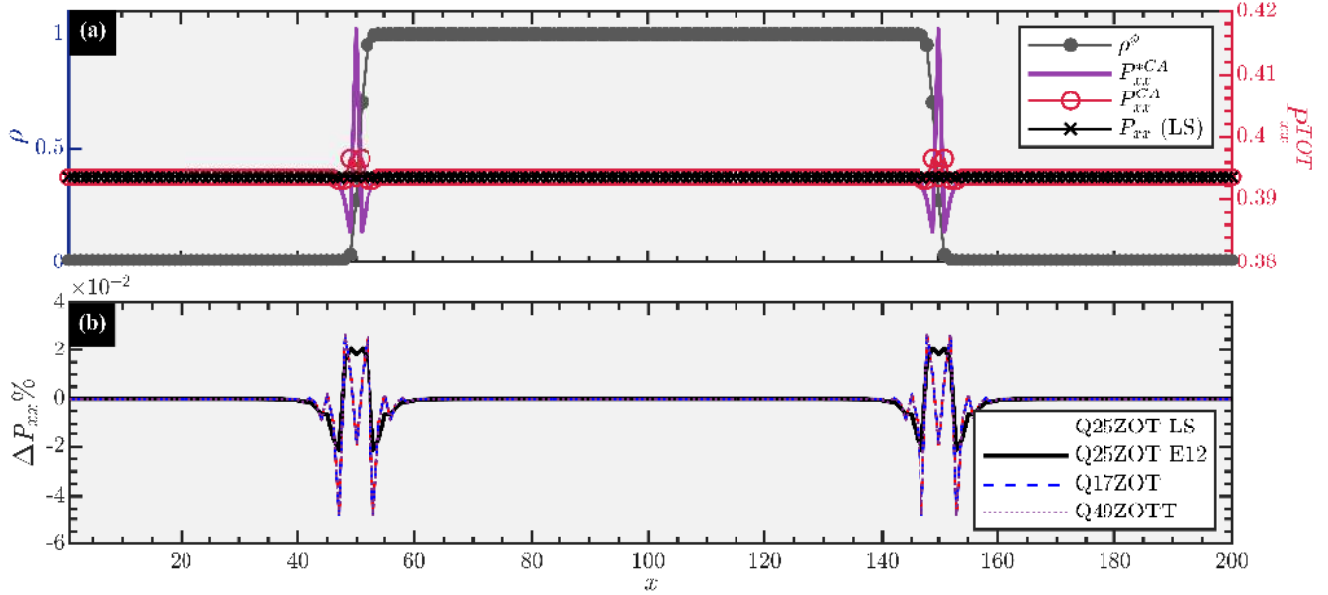
FIG. 6: Numerical results at equilibrium for the flat interface test for a variety of lattice structures. (a) Pseudopotential interactions (11) are deployed directly on the Q25ZOT lattice structure. The interaction component of P_{xx}^{TOT} obtained numerically P_{xx} ( \times ) from Eq. (17) and its continuum approximation P_{xx}^{CA} ( \circ ) from Eqs. (29) and (30) are compared against the standard solution P_{xx}^{*CA} (solid line) from Eq. (19). (b) Constancy \Delta P_{xx}/\% of the P_{xx} obtained numerically with Eq. (17) along spatial dimension x , tested for Q25ZOT on the LS and with E12, in addition to Q17ZOT and Q49ZOTT. Here, for Q49ZOTT, the sound speed c_s was modified to match that of the ZOT variants.
