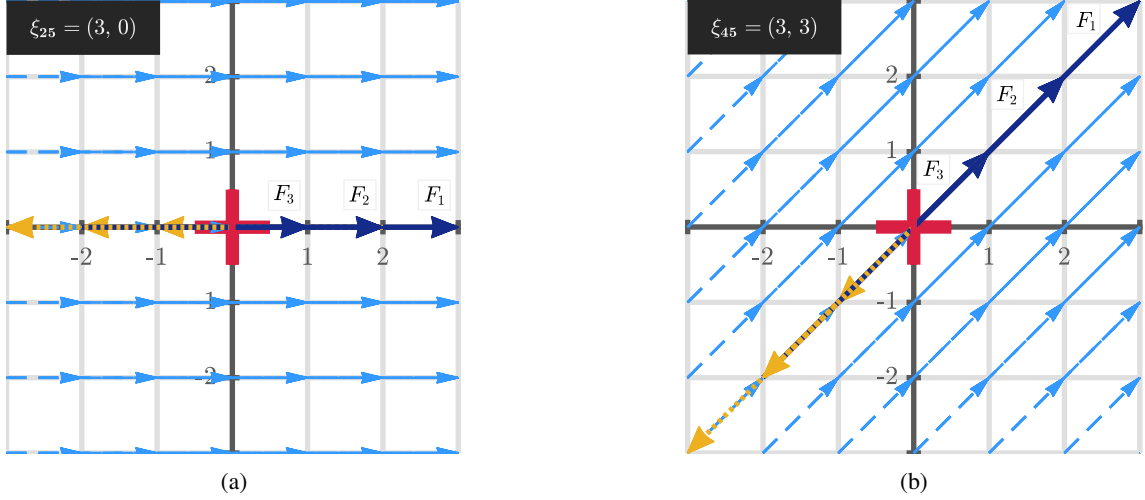
FIG. 2: Illustration of the force vectors along the vectors \xi_\alpha that belong to symmetry group \bar{z} and pass through (bold solid arrows) the infinitesimal horizontal d\mathbf{A}^{(x)} and vertical d\mathbf{A}^{(y)} unit area elements (bold red line) centered at \mathbf{x} . In reference to the Q49ZOTT lattice in Fig. 1, force vectors along (a) \xi_{25} ( \bar{z} = 9 ) and (b) \xi_{45} ( \bar{z} = 18 ) are shown. In both cases, there is a total of six ( 2\mathcal{E}^z ) force vectors contributing equally to their respective interaction pressure tensor, i.e., \mathcal{P}_{ij}^{int, \bar{z}=9} and \mathcal{P}_{ij}^{int, \bar{z}=18} . The six force vectors consist of four different classes of vectors; one ( F_1 ) starts and another ends (accounted for along the opposite, \xi_a ) at \mathbf{x} , and two ( F_2 and F_3 ) pass through \mathbf{x} . Labeled force vectors are those to be explicitly considered along each respective \xi_\alpha . The unlabeled bold dotted arrows are not considered along vectors \xi_\alpha but are instead accounted for along the opposite \xi_a (hence the direction of arrows) as a result of symmetry and summation around the lattice, for example, in this case (a) \xi_{27} and (b) \xi_{47} . These are automatically considered in Eq. (15).
