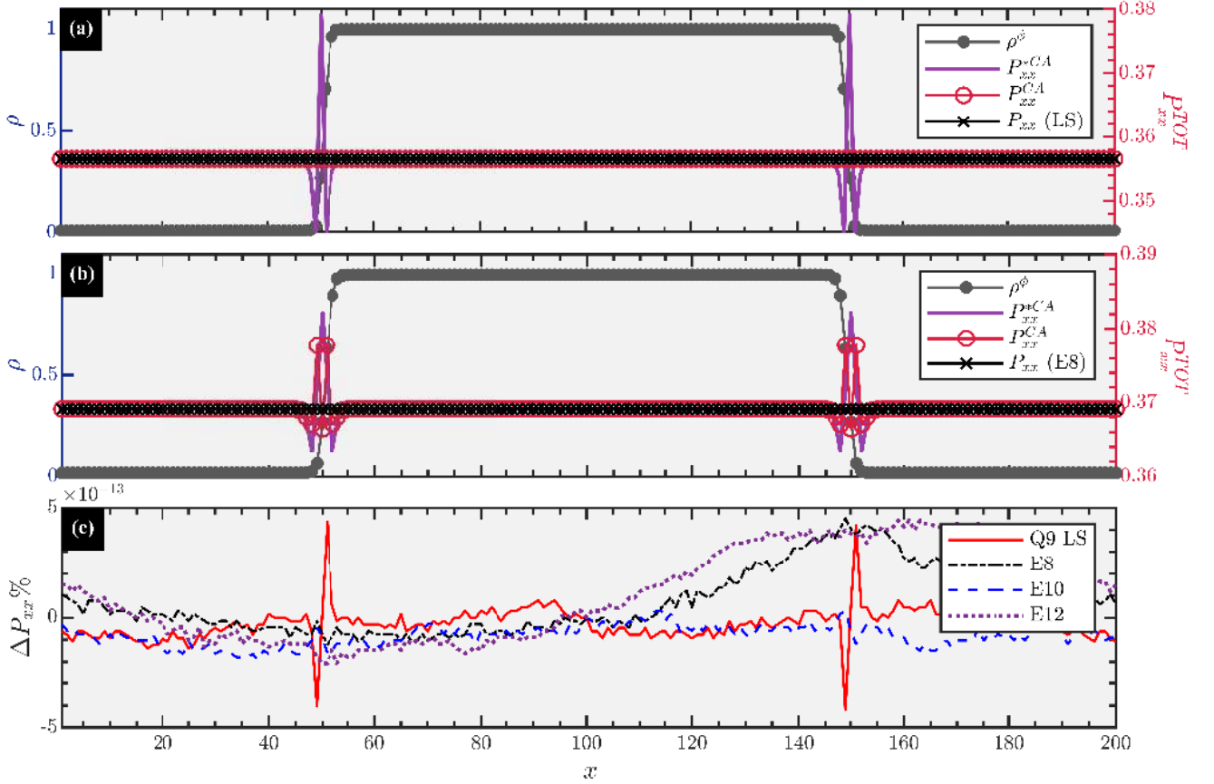
FIG. 5: Numerical results at equilibrium for the flat interface test using the Q9 lattice model. The pseudopotential interactions (11) are deployed (a) directly on the lattice structure (LS) and (b) with the E8 model. The interaction component of P_{xx}^{TOT} obtained numerically P_{xx} ( \times ) from Eq. (17) and its continuum approximation P_{xx}^{CA} ( \circ ) obtained from Eqs. (29) and (30) are compared against the standard solution P_{xx}^{*CA} (solid line) from Eq. (19). (c) Constancy \Delta P_{xx} \% of the P_{xx} obtained numerically (17), tested for the Q9 LS, E8, E10, and E12 along spatial dimension x . For each lattice, the constancy \Delta P_{xx} \% is calculated as the percentage difference of P_{xx} along x against the reference P_{xx}(x) measured at center x = 100 .
