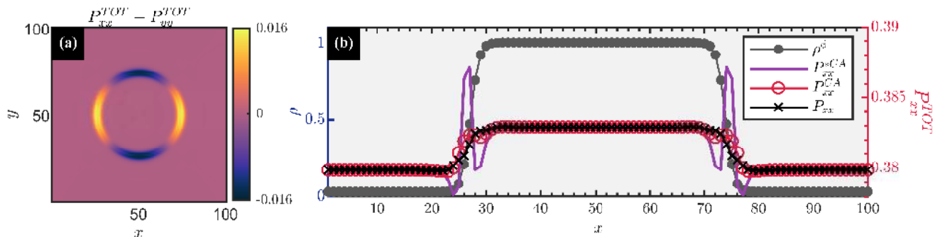
FIG. 7: (Color online) Single static circular droplet results for Q49ZOTT* with modified c_s . (a) Mismatch between normal and tangential components of the total pressure tensor (9), (10), and (17). (b) Cross-sectional profiles along x at y = n_y/2 , comparing the interaction component of P_{xx}^{TOT} obtained numerically P_{xx} ( \times ) from Eq. (17), its continuum approximation P_{xx}^{CA} (c) from Eqs. (29) and (30) and the standard solution P_{xx}^{*CA} (solid line) from Eq. (19).
