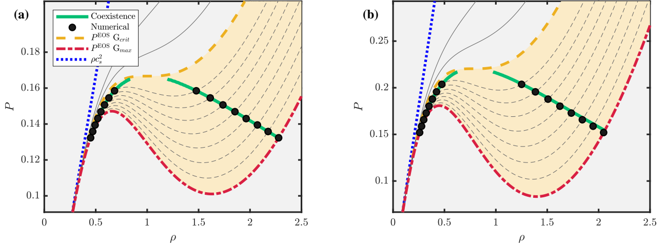
FIG. 4: Theoretical prediction of equation of state P_o (dashed and dotted curved lines) for a range of \mathcal{G}/\mathcal{G}_{crit} up to \mathcal{G}_{max} = \mathcal{G}_{crit} \cdot 1.225 (red dot-dashed line), solved for (a) the Q9 lattice model ( \epsilon = 0 ) with \psi(\rho) = e^{-1/\rho} and (b) the Q49ZOTT lattice model with Eqs. (30) and (35). The thermodynamic coexistence curve (bold solid green line) drawn within the shaded region is obtained from the Maxwell construction (34). Numerical simulations were conducted for \mathcal{G}/\mathcal{G}_{crit} = \{1.05, 1.075, 1.1, 1.125, 1.15, 1.175, 1.2, \mathcal{G}_{max}\} where the bulk properties of each phase ( \bullet ), namely, densities and corresponding static pressure, are obtained from Eqs. (7a), (9), and (17).
