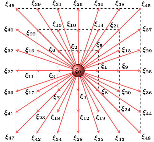
FIG. 1: Two-dimensional high-order lattice model constructed from projection of D1Q7 [37], i.e., a total of 7^2 = 49 lattice velocities. We denote this lattice structure by Q49ZOTT, based on its D1Q7 construction on zero-one-two-three (ZOTT) velocity, analogous to the zero-one-three (ZOT) construction used for D2Q25ZOT in [37]. Refer to Appendix A for details.
