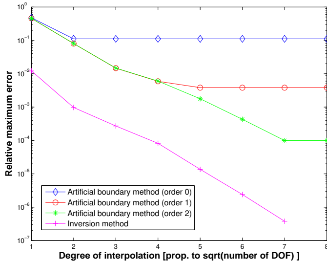
Figure 6: Comparison inversion method / absorbing boundary condition.
