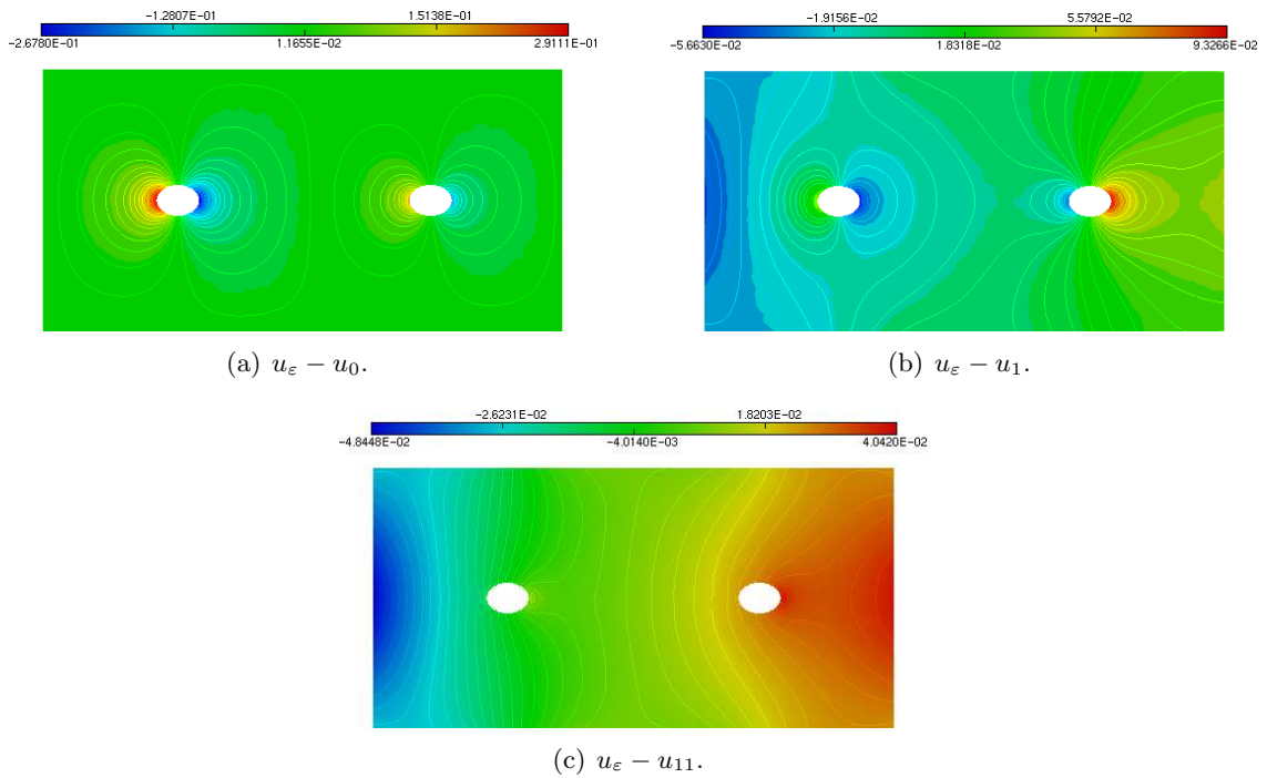
Figure 9: u_\varepsilon - u_0 and u_\varepsilon - u_1 for \varepsilon = 0.0585 and \alpha = 0.5 .
