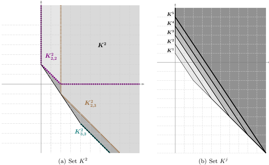
Figure 4: The sets of indices
