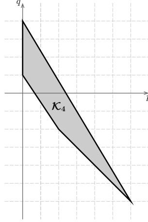
Figure 2: The set of indices \mathcal{K}_4 for \alpha = \frac{3}{5} .
