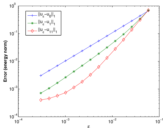
Figure 10: Energy norms of u_\varepsilon - u_0 , u_\varepsilon - u_1 , and u_\varepsilon - u_{11} . for \alpha = 0.2 .
