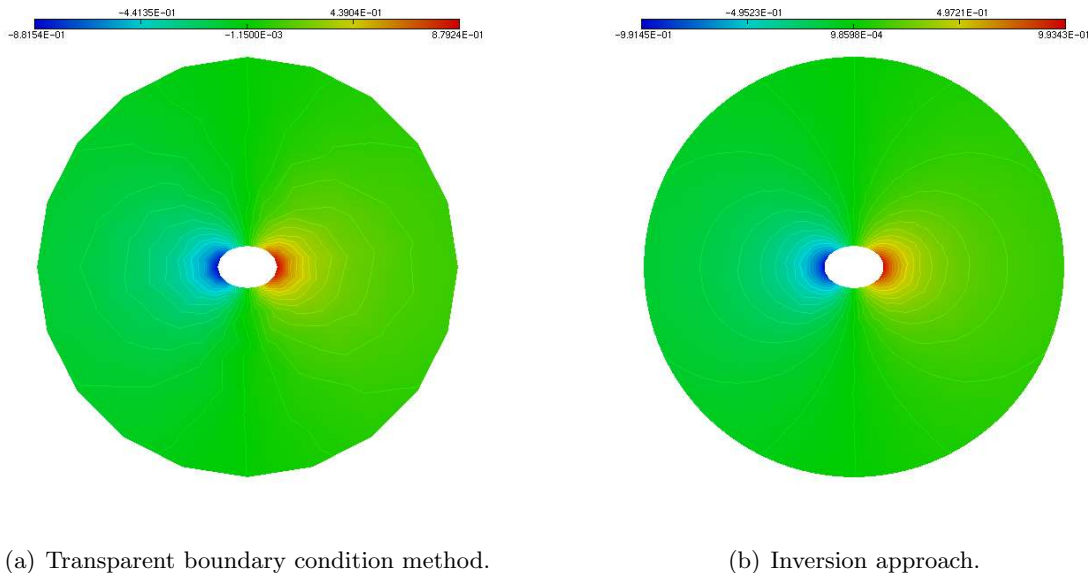
Figure 7: Profile obtained for the same number of DOF.
