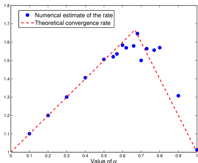
Figure 11: Predicted and estimated convergence rate with respect to \alpha .
