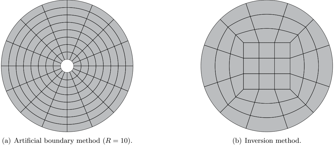
Figure 5: Meshes used for the computation of the profiles
