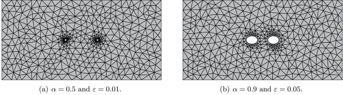
Figure 8: Some meshes used to compute u_\varepsilon .
