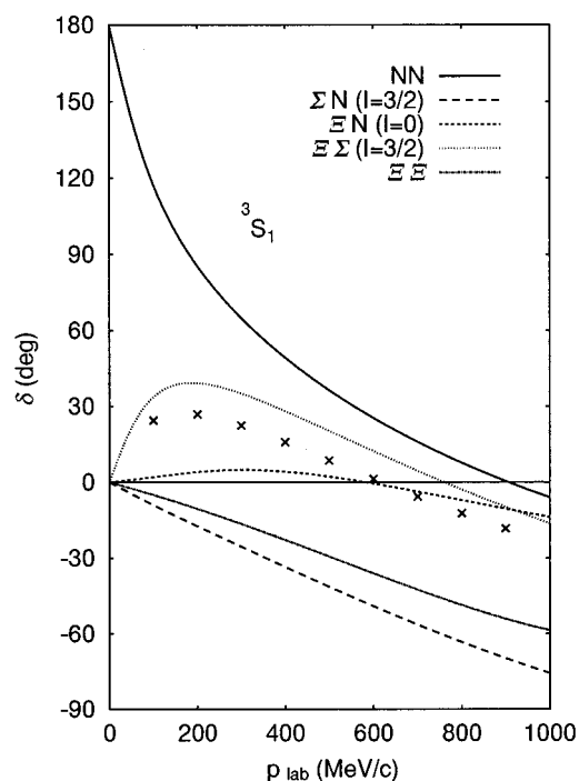
FIG. 2. ^3S_1 phase shifts for the (03) [ NN , \Xi\Sigma(I=3/2) ], (11)_a [ \Xi N(I=0) ], and (30) [ \Sigma N(I=3/2) , \Xi\Xi ] states. The ^3S phase shift predicted only by the NN central interaction is also shown by crosses.
