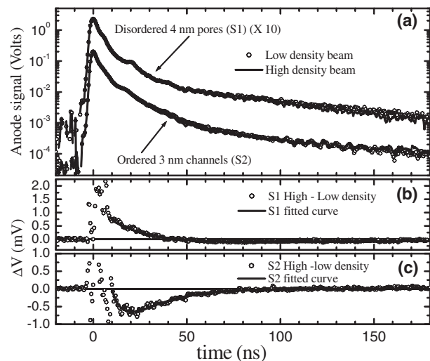
FIG. 1. (a) Lifetime spectra at room temperature using samples S1 and S2 taken at low ( S1 = 9.5 \times 10^9 cm -2 , S2 = 6.7 \times 10^9 cm -2 ) and high ( S1 = 2.9 \times 10^{10} cm -2 , S2 = 2.5 \times 10^{10} cm -2 ) beam areal densities. The S1 data are displaced (by a factor of 10) for clarity. The bump in the curves at about 19 ns is due to light feedback in the PMT, and smaller wiggles at later times are caused by internal cable reflections. (b–c) Difference between the high and low density data for S1 and S2, respectively, and the fits (as described in the text) from which the parameters \beta_{S1} and \beta_{S2} were obtained.
