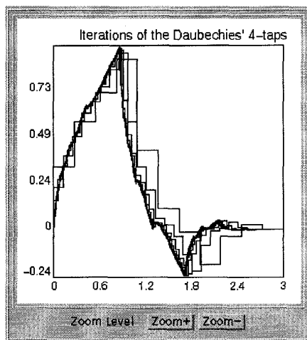
Figure 4: Iterations of the 4-tap Daubechies filter
