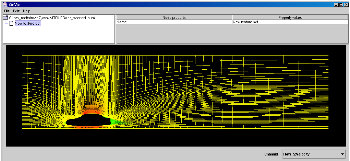
Figure 5: Air-Flow around a moving car: After loading the data set, an empty feature set is created, and the spatial layout of the data is shown, overall velocity information is mapped to color (green denotes low, red high velocity).
