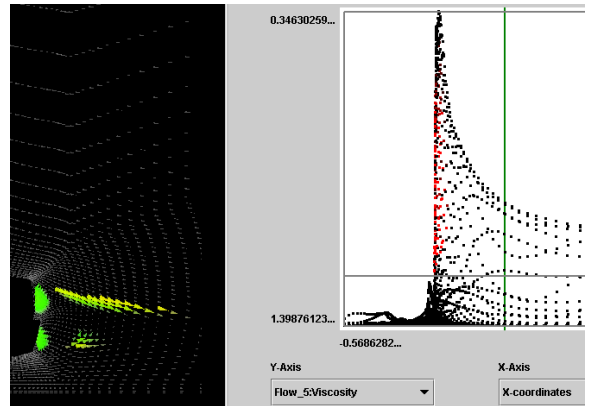
Figure 7: Step 2 of analysis: AND-refinement, restricting feat. spec. to high viscosity values in the second scatterplot view. Only features behind the car are part of focus now.
