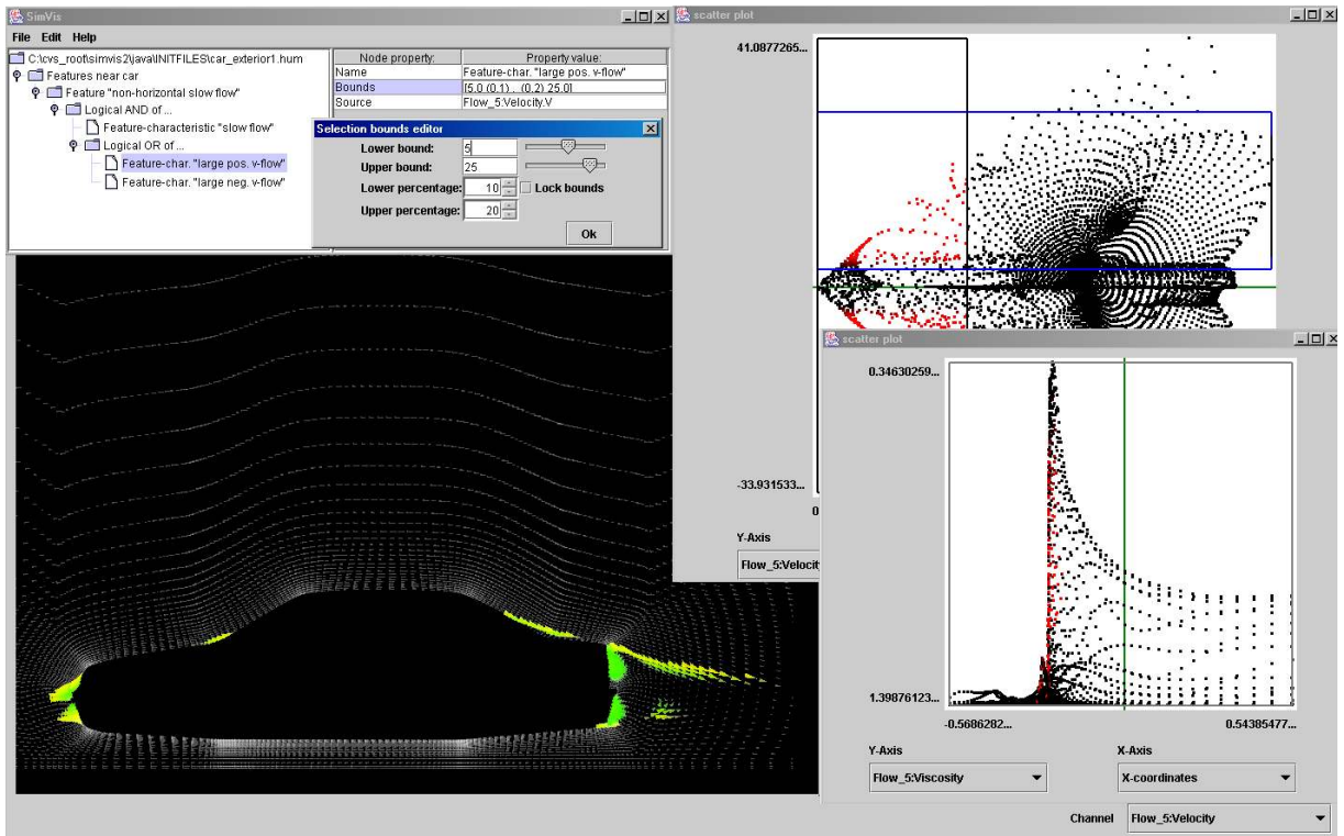
Figure 6: First step of analysis (non-horizontal slow flow): a tree viewer showing the current feature specification in the upper left (interaction panel for adjusting a simple feature characteristic shown), a scatterplot view used for feature specification in the upper right (velocity vs. V-Velocity component), the SciViz view for f+c visualization in the lower left, a second scatter plot for visualization of f+c distribution (X-coordinates vs. viscosity).
