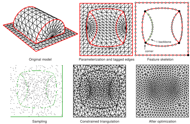
Figure 6: Simple example of features: the feature edges (in red) are chained together to create the feature graph; a 1D error diffusion is then performed along the graph followed by a constrained Delaunay triangulation of the whole sampling; after a constrained mesh optimization, the feature edges are perfectly preserved, while blended in the new mesh.
