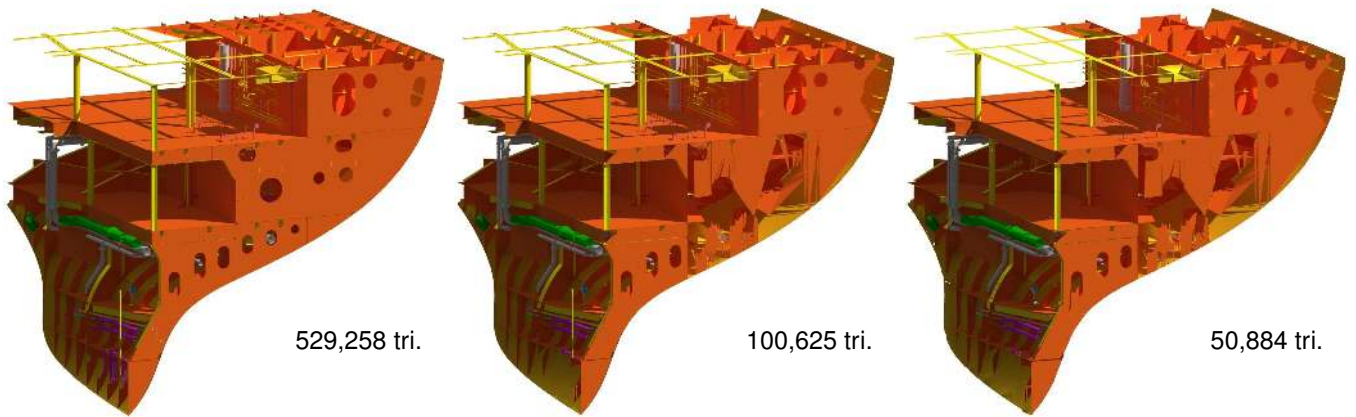
Figure 3: Node simplification: The leftmost image shows the exact geometry corresponding to one of the nodes in the Kd-tree. In the center image, some of this geometry has been removed by the visibility culling (which is conducted including geometry from neighboring nodes, since the simplified versions are not meant to be used from close-up). The rightmost image shows the result of the simplification of this node. Notice that there are large holes in the front wall; they happen because those portions of the wall are occluded by geometry in the neighboring node, and will therefore never be visible when this simplification is used.
