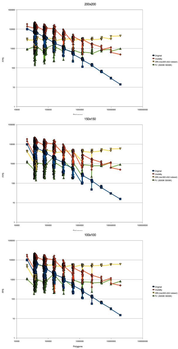
Figure 6: Comparative speeds in different rendering techniques for large datasets in a 200 \times 200 viewport (top), a 150 \times 150 viewport (middle) and a 100 \times 100 viewport. The test was run on a machine with a 4-core intel i7 at 3.2Ghz, with 12Mb of memory and a GeForce GTX570 graphics card with 1.25Gb of DDR5 memory, using Windows 7 Professional 64bits.
