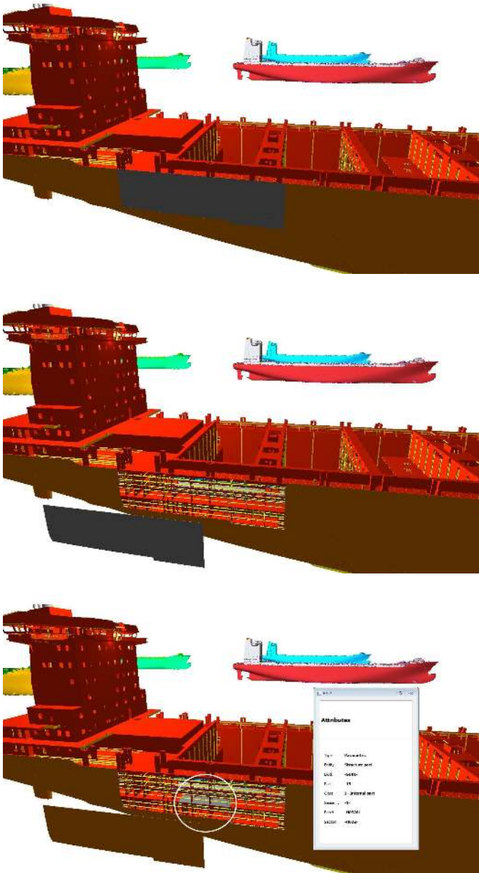
Figure 1: The model used in the tests. The top image shows a portion of the hull selected by the user in gray. In the middle image the user has moved the selected portion of the hull, partially revealing the complexity of the model inside. The bottom image shows data associated to an object, that the user may annotate. Notice the ships in the background, which are rendered using omnidirectional relief impostors
