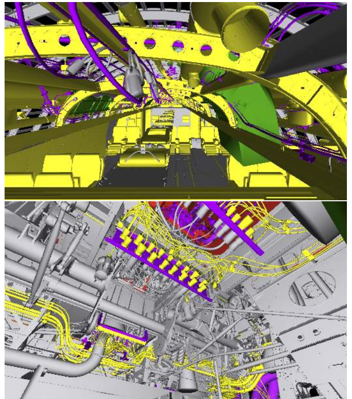
Figure 5: Two frames from a navigation inside the Boeing 777-200. The top frame shows a view near the top of the cabin, where sight extends all the way to the rear end of the airplane. Notice that upon careful inspection, far elements, rendered as ORIs, can be distinguished as slightly more blurred. Nodes at a mid-distance are simplified, and geometry close to the camera is exact. The bottom figure shows a frame where we see that the model has preserved intact the detail of the original for close inspection.
