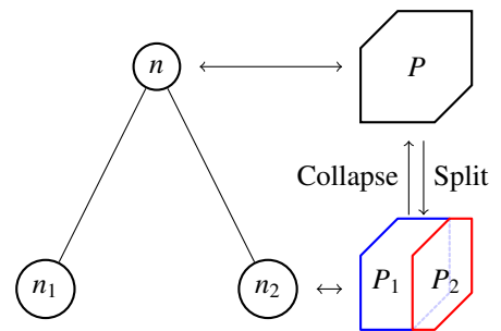
Figure 2: Base Visual contribution is monotonic. The Split operation increases it, while the Collapse operation decreases it.
