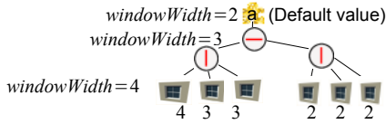
Figure 8: On every shape we can assign values to variables. Assignments extend their scope to all underlying shapes. Assignments on lower levels override assignments on higher levels. Numbers below windows show the values of windowWidth .
