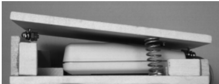
Fig. 2-2. Side view of the “footmouse.” Note the small screws used to depress the mouse buttons.
