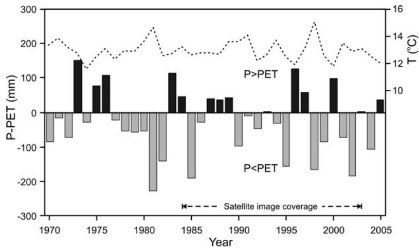
Figure 2. Interannual climate variability for the Utikumma Uplands. The climate data were compiled for the Whitefish Lookout station (56°10'N, 115°28'W; 610 m asl), which recorded climate data from May to August only. T, growing season average of daily mean air temperature; P – PET, growing season total of daily total precipitation minus daily total potential evapotranspiration.
