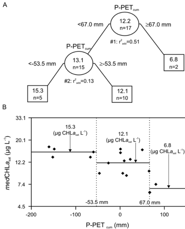
Figure 5. (a) Regression tree and (b) corresponding annotated scatterplot quantifying the relation between landscape median (Chl a ) sat and growing season total of daily total precipitation minus daily total potential evapotranspiration ( P - PET_{cum} ). The model explained 64% of the total variance in (Chl a ) sat . In Figure 5a, ovals and rectangles represent splitting and terminal nodes, respectively, and numbers within node symbols indicate average (Chl a ) sat ( \mu\text{g L}^{-1} ) (back transformed using exponential function) and sample size of that node.
