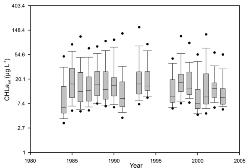
Figure 3. Wit - d among-year variability of (Chl\ a)_{sat} from 1984 to 2003 (1992, 1995, and 1996 are missing because o ack of suitable imagery). Note log scale for y axis.
