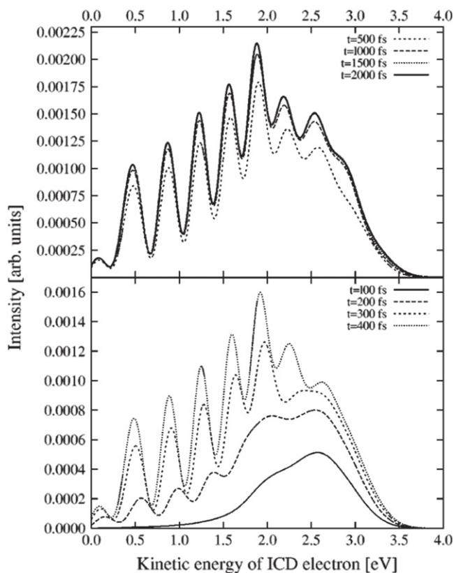
Figure 14. Temporal evolution of the kinetic energy spectrum of the ICD electron. After a certain time the nodal structure of the decaying intermediate vibrational wave packet becomes clearly visible with the spectrum converging at times of approximately 2 ps. Reprinted with permission from [15]. Copyright 2003, AIP Publishing LLC.
