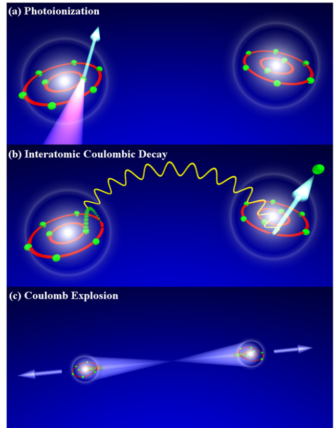
Figure 1. Interatomic Coulombic decay in a neon dimer: (a) A 2s-inner-valence-electron is removed from one atom of a neon dimer. (b) As the vacancy is filled by a 2p-electron the energy gained is transferred to the other atom of the dimer in a dipole/dipole-interaction. (c) As two singly charged neon ions are facing each other after the decay, the dimer fragments in a Coulomb explosion. The process sketched in (b) corresponds to the ‘direct’ contribution to ICD (see text). Reprinted with permission from [3]. Copyright 2004 by the American Physical Society.
