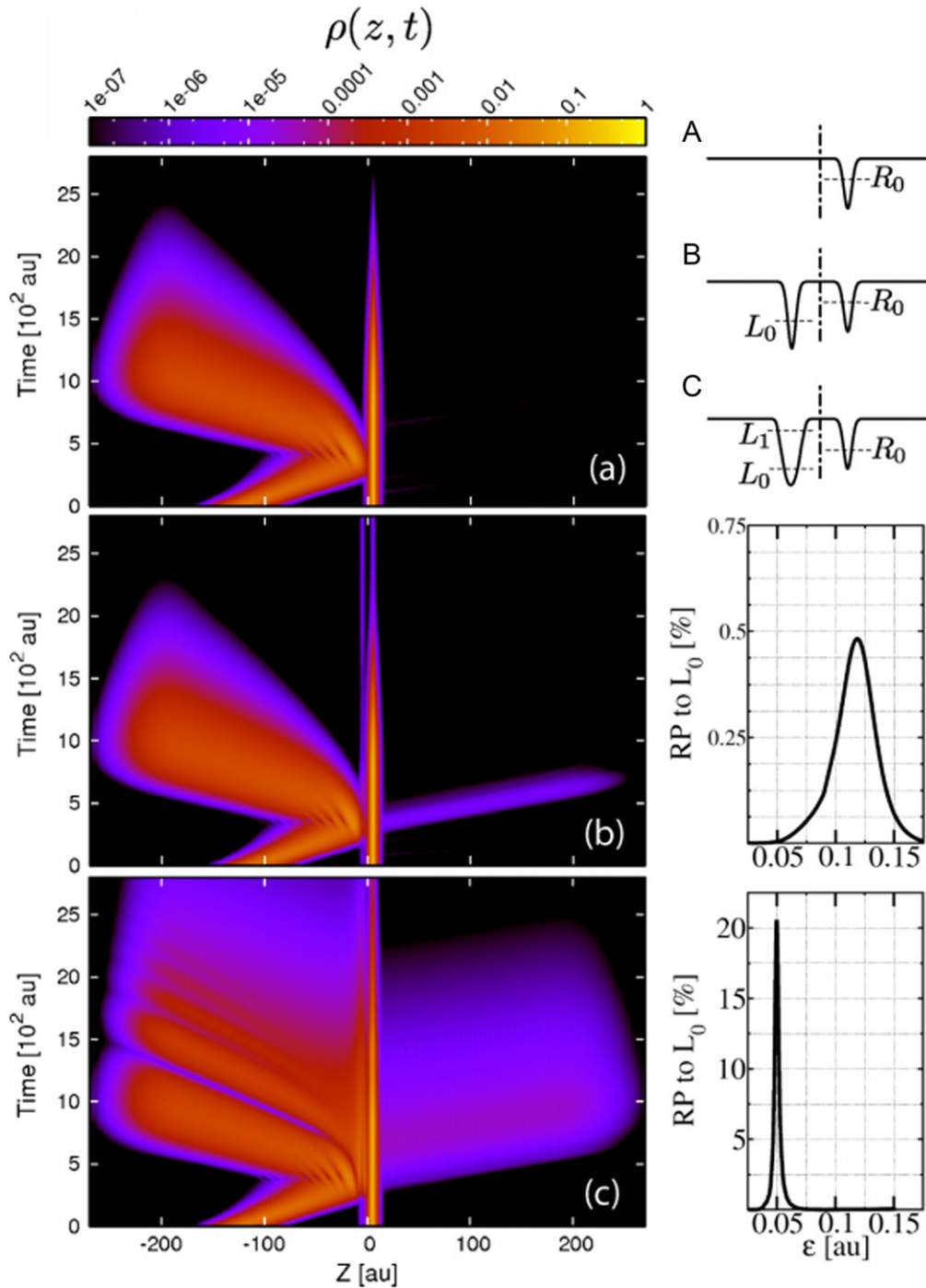
Figure 9. Temporal evolution of the electron density for the three setups shown in the upper right corner. On the right the corresponding reaction probability (RP) in dependence of the incident energy \epsilon is depicted. Reprinted with permission from [81]. Copyright 2013 by the American Physical Society.
