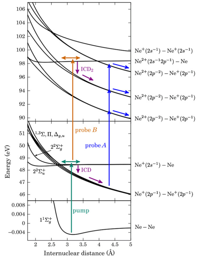
Figure 21. Potential energy surfaces of the neon dimer that are involved in the pump/probe scheme by Schnorr et al to extract the lifetime of single ICD events. Reprinted with permission from [148]. Copyright 2013 by the American Physical Society.
