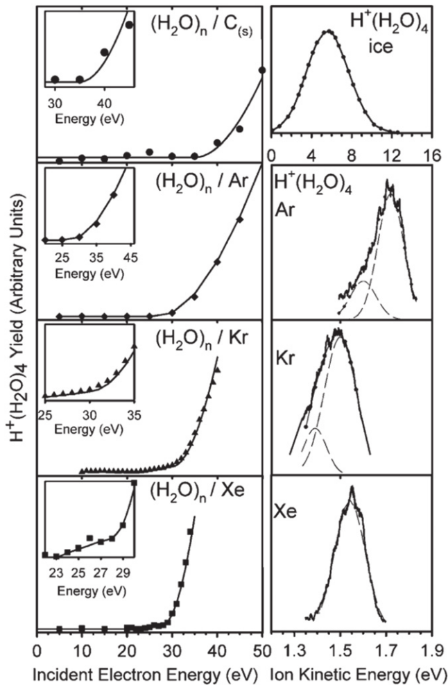
Figure 8. Evidence for ICD at heterogenous interfaces. (Left) Incident electron kinetic energy versus cluster ion yield for monolayer water films of water on graphite, Ar, Kr and Xe. (Right) Kinetic energy of the emitted \text{H}^+(\text{H}_2\text{O})_4 ions for the different substrates. Reprinted with permission from [76]. Copyright 2011 by the American Physical Society.
