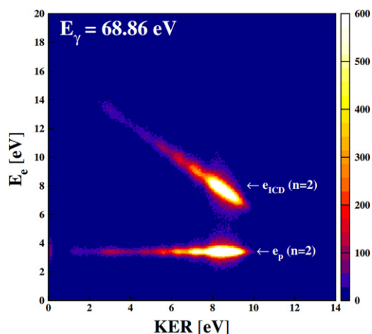
Figure 18. Kinetic energy release versus electron kinetic energy of a Coulomb exploding He dimer. Reprinted with permission from [31]. Copyright 2010 by the American Physical Society.
