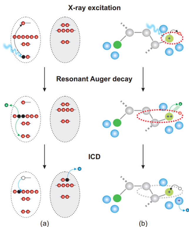
Figure 5. (a) ICD after resonant Auger decay. (b) The parent state of ICD is exclusively created at a certain atom of an embedded system, as this atom is excited resonantly. Reprinted with permission from [63]. Copyright 2013, rights managed by Nature Publishing Group.
