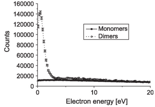
Figure 7. Kinetic energy of the electrons emitted from neon monomers (solid squares) and neon dimers (open circles) after collision with a 0.65 \text{ MeV He}^+ projectile. Reprinted with permission from [72].
