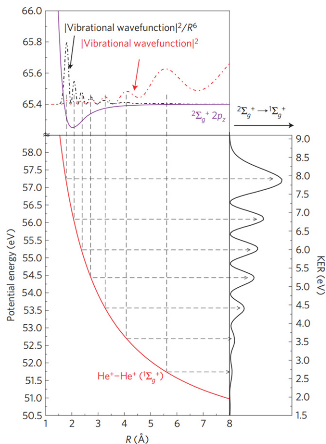
Figure 20. Top: probability density of the vibrational wave function of the electronic state that is mainly populated in the initial shakeup process ( 2^2\Sigma_g^+ 2p_z ) (red dotted line). The black dotted line shows the latter probability density multiplied with 1/R^6 taking into account the decay behavior. Middle: potential energy curve of the final state of the decay. Right: kinetic energy release after the decay. Reprinted with permission from [144]. Copyright 2010, rights managed by Nature Publishing Group.
