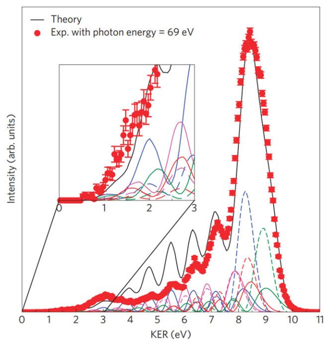
Figure 19. Kinetic energy release of the Coulomb exploding He dimer after ICD. The theoretical spectrum (black line) was obtained by adding up all partial spectra (colored lines). Reprinted with permission from [144]. Copyright 2010, rights managed by Nature Publishing Group.
