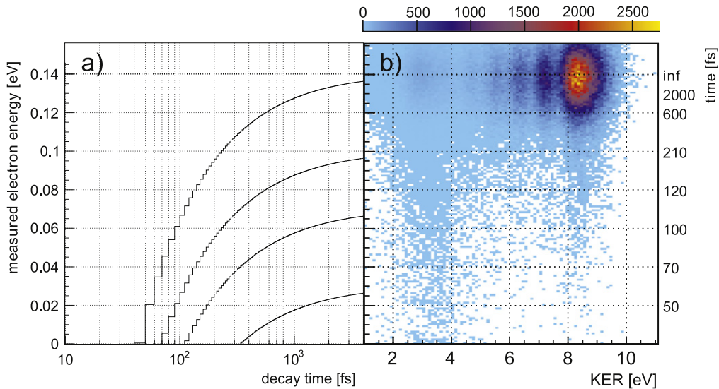
Figure 22. (a) Conversion of measured photoelectron energy to decay time: the four lines show four examples of initial (undisturbed) photoelectron energies of (top to bottom) 140, 100, 70 and 30 meV. If, for example, an electron that is expected to occur at an energy of 140 meV is decelerated due to PCI (see text) and measured at an energy of 60 meV the corresponding decay time was 100 fs. (b) KER versus measured electron energy. The time-axis on the right was obtained according to the most upper curve (initial energy of 140 meV). Reprinted with permission from [149]. Copyright 2013 by the American Physical Society.
