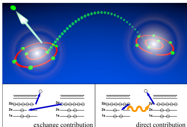
Figure 2. Top: the exchange contribution to interatomic Coulombic decay. Bottom: involved energy levels for the case of ICD of a neon dimer, showing the exchange contribution (left) and the aforementioned direct contribution (right).
