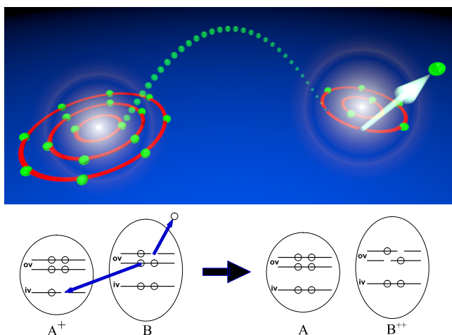
Figure 10. Sketch of ETMD(2). Top: an inner-valence vacancy in a heteronuclear dimer is filled by an electron from a neighboring atom. The excess energy is used to emitted a further electron from that atom. Bottom: representation depicting the inner-valence (iv) and outer-valence (ov) energy levels involved in ETMD(2). After ETMD(2) the atom A is neutralized, while atom B is doubly charged (right).
