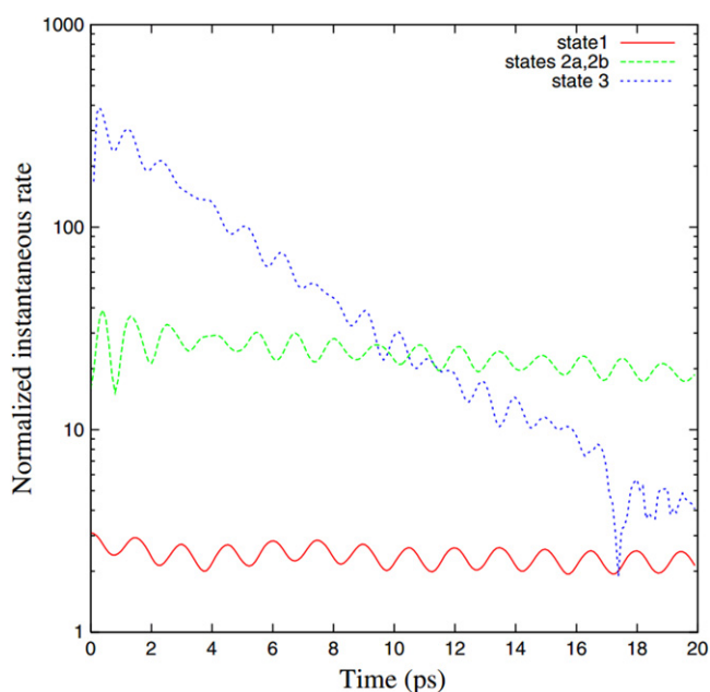
Figure 17. The normalized instantaneous rate of the decay states 1, 2a, 2b and 3 (see text) as a function of time. Reprinted with permission from [129]. Copyright 2010 by the American Physical Society.
