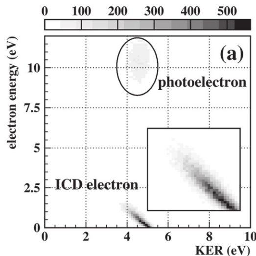
Figure 3. Unambiguous proof for ICD in a neon dimer. Reprinted with permission from [3]. Copyright 2004 by the American Physical Society. As the sum of the kinetic energy release and the ICD electron kinetic energy is a constant, events of ICD occur in this representation as a diagonal feature.
