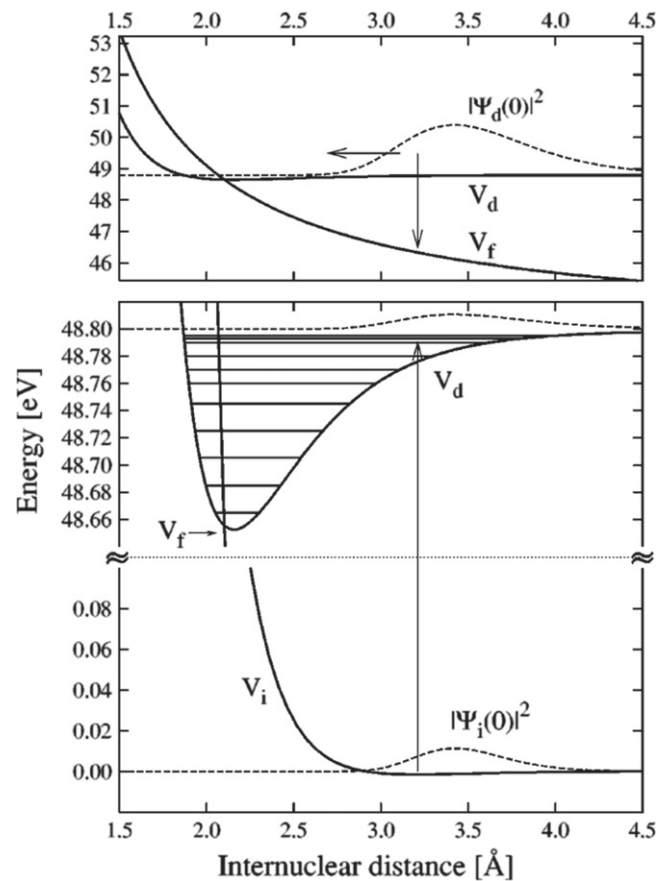
Figure 13. Visualizing the role of nuclear dynamics of ICD: a neon dimer is ionized from the ground state ( V_i ) to the intermediate state ( V_d ) that will undergo ICD (lower panel). After population the intermediate wave packet starts to propagate and decay to the final state ( V_f ) (upper panel). Reprinted with permission from [15].
