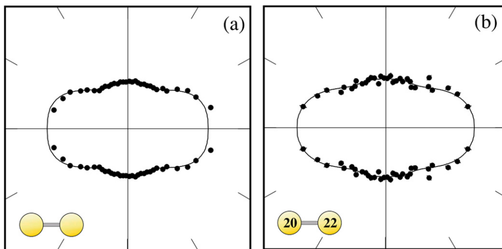
Figure 16. Angular emission pattern of the ICD electron in the dimer frame. The dimer is aligned horizontally, as depicted by the icon. (a) shows the emission distribution for ^{20}\text{Ne}^{20}\text{Ne} and (b) for ^{22}\text{Ne}^{20}\text{Ne} . Reprinted with permission from [127].
