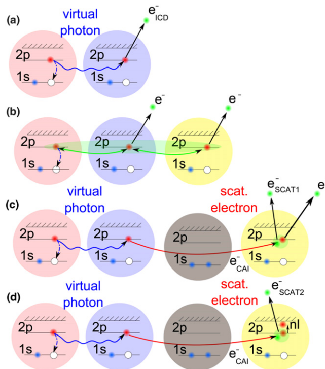
Figure 12. Depending on the amount of (excited) surrounding atoms many different interatomic de-excitation mechanisms are possible and were observed in [121]: (a) ICD of the multiply excited constituents, (b) ‘collective autoionization’ (CAI) of three or more excited atoms and (c), (d) a CAI involving scattering of the emitted electron. Reprinted with permission from [121]. Copyright 2014 by the American Physical Society.
