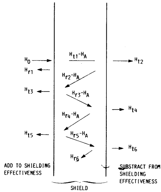
FIGURE 4. - MULTIPLE REFLECTIONS OF A MAGNETIC FIELD WITHIN A SHIELD WHERE H_0 IS THE INCIDENT FIELD, H_A IS THE ABSORPTION OF THE SHIELD, H_{tn} IS THE TRANSMISSION THROUGH THE "n TH " REFLECTED WAVE AND H_{rn} IS THE REFLECTION THROUGH THE "n TH " REFLECTED WAVE.
