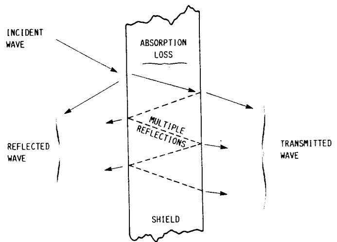
FIGURE 2. - SHIELDING EFFECTIVENESS.
