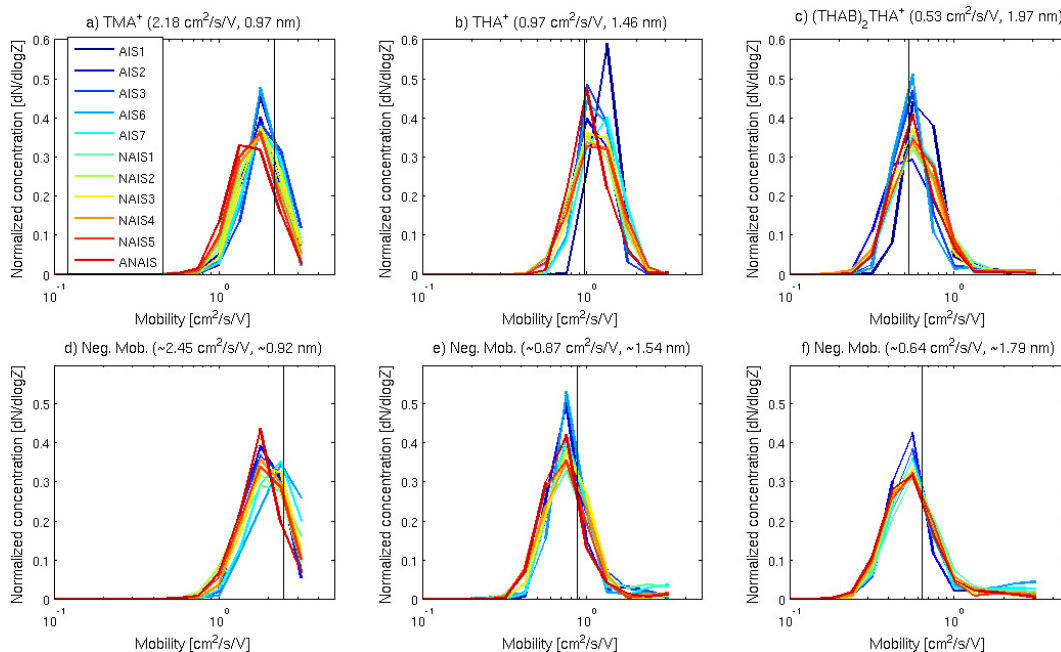
Fig. 1. Examples of mobility standards measurements. Subfigures (a) , (b) and (c) show the response of the ion spectrometers (normalized mobility distribution) for 3 positively charged mobility standards, and subfigures (d) , (e) and (f) for 3 negative mobilities. The black vertical lines represent the mobility that was selected through the HDMA. The mobility and size of the standards are above each plot. TMAI is tetra-methyl ammonium iodide and THAB is tetra-heptyl ammonium bromide.
