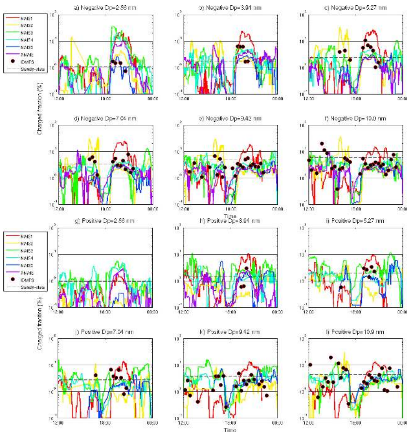
Fig. 7. Negative (a to f) and positive (g to l) charged fraction (fraction of charged particles in percents) at 6 different diameters as a function of time for all NAISs on 12 June 2009. The charged fraction retrieved with the Ion-DMPS is shown as black circles and the bipolar steady-state charged fraction is marked with a black dashed line.
