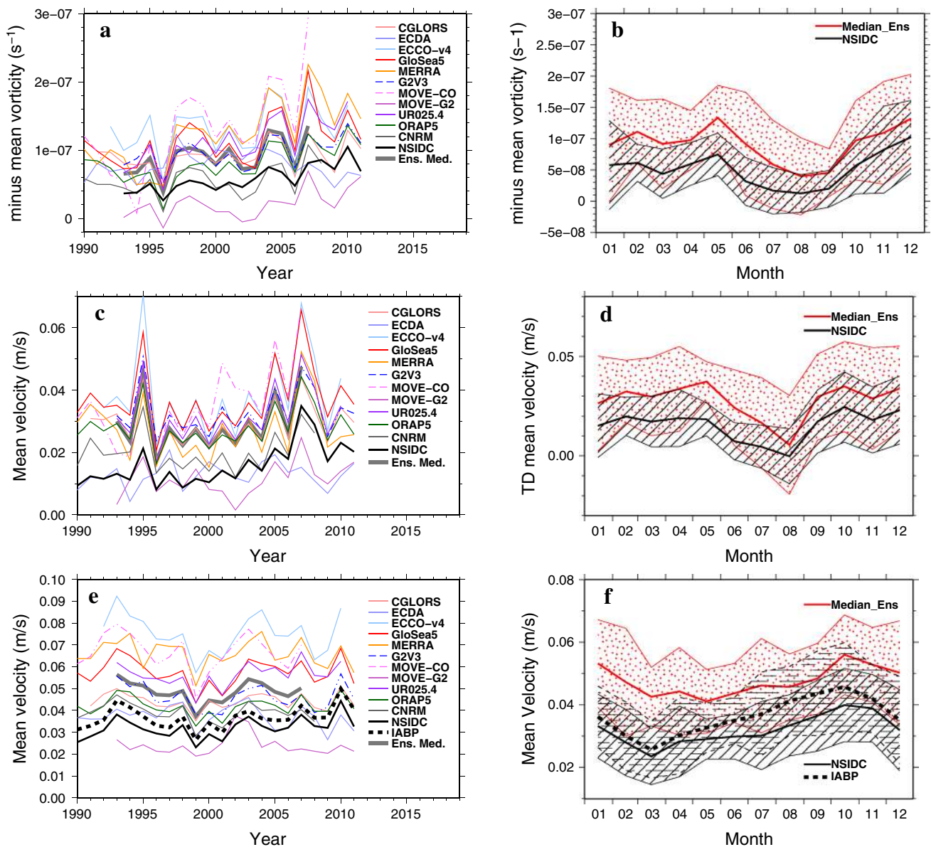
Fig. 11 a Annual vorticity (sign reversed, s^{-1} ) averaged over a sector (from 73^{\circ}\text{N} to 82^{\circ}\text{N} in latitude and from 175^{\circ}\text{E} to 135^{\circ}\text{W} in longitude) covering the Beaufort gyre for the different members of the ensemble, the median of the ensemble and the NSIDC product used as a reference. b Seasonal cycle for the mean vorticity for the median of the ensemble (thick red) and the NSIDC product (thick black) over the 1993–2007 period. Regions delimited by thin red and black lines and filled with red dots and black slanted patterns indicate the mean plus or minus one standard deviation for each month for the two
