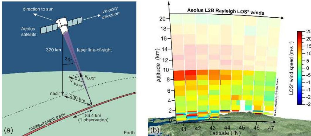
Figure 5. (a) Aeolus observational geometry, and (b) Aeolus L2B LOS* Rayleigh winds (positive if winds are blowing away from the instrument) measured during the underflight on 22 November 2018 between 40.6 and 47.2° N. Only winds with an estimated wind error of less than 12 m s -1 are shown. Winds at altitudes above 10 km are outside of the measurement range of the A2D and are consequently greyed out. The figure was created based on a screenshot from the Aeolus data visualization tool, © VirES for Aeolus ( https://aeolus.services/ , last access: 25 November 2019).
