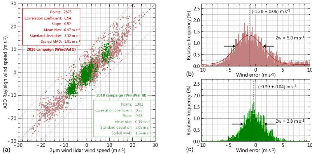
Figure 6. (a) Scatterplots comparing the A2D Rayleigh LOS winds with the 2 µm DWL winds for all Aeolus underflight legs from the WindVal III campaign in 2018 (green) and for all flights from the WindVal II campaign in 2016 (red). The corresponding probability density functions for the wind differences (A2D–2 µm), i.e. the A2D wind error, are shown in panels (b) and (c) for the two campaigns respectively. The solid lines represent Gaussian fits with the given centres and e^{-1/2} widths 2w .
