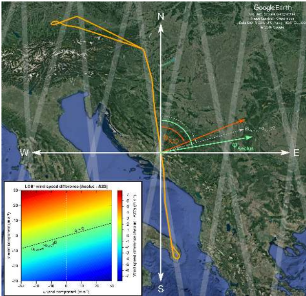
Figure 8. Diagram illustrating the different azimuth angles of Aeolus (green arrow) and the A2D (orange arrow), using the underflight on 22 November 2018 (indicated by the orange flight track) as an example (background image: © 2018 Google). The inset depicts the dependence of the LOS* wind speed difference on the zonal ( u ) and meridional ( v ) wind components for azimuth angles of \varphi_{A2D} = 68 and \varphi_{Aeolus} = 80^\circ . When the azimuth angle of the wind vector meets the condition \varphi_{wind} = (\varphi_{Aeolus}/\varphi_{A2D})/2 , i.e. the wind direction is 74^\circ (dashed grey arrow), the LOS* wind speed difference \Delta is zero.
