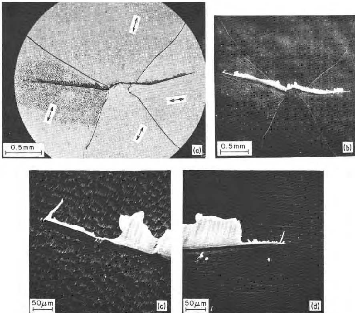
Figure 5 First crack produced in ice at -10^{\circ}\text{C} under a stress of 1\text{ MN m}^{-2} . (a) optical micrograph of the replica. Arrows indicate direction of [0001] axis. (b) Scanning electron micrograph of the same replica. (c) and (d) SEM of the crack tip areas.
