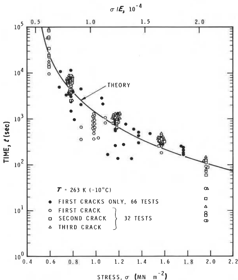
Figure 2 Dependence of time to the formation of first cracks on stress, T = 263 \text{ K} (-10^\circ \text{ C}) . Experimental results are from Gold [28, 29].
