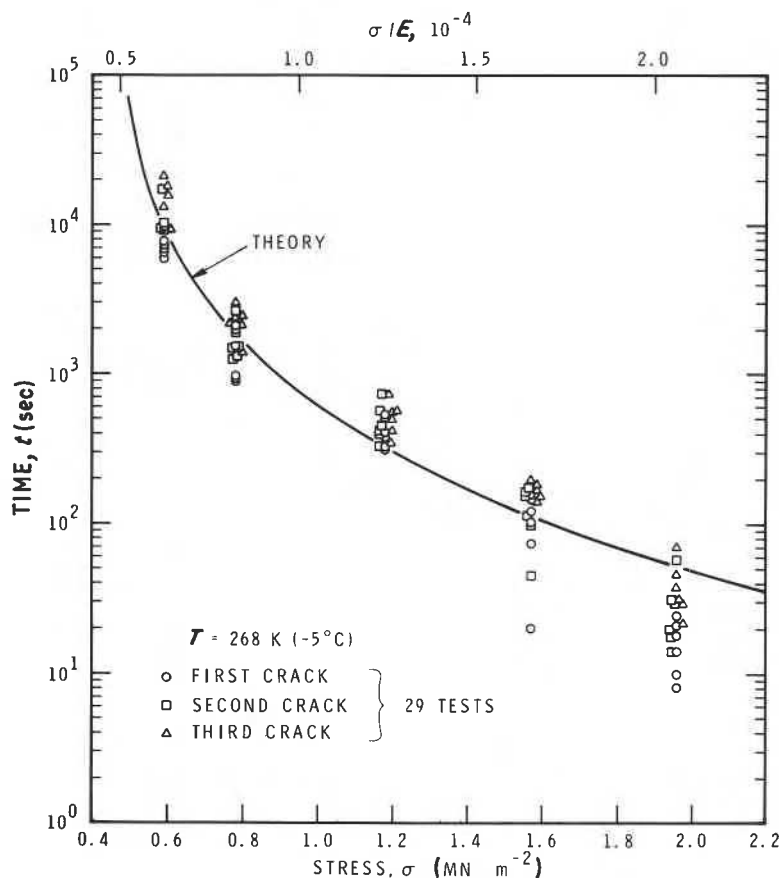
Figure 1 Dependence of time to the formation of first cracks on stress, T = 268 \text{ K} (-5^\circ \text{ C}) . Experimental results are from Gold [28, 29].
