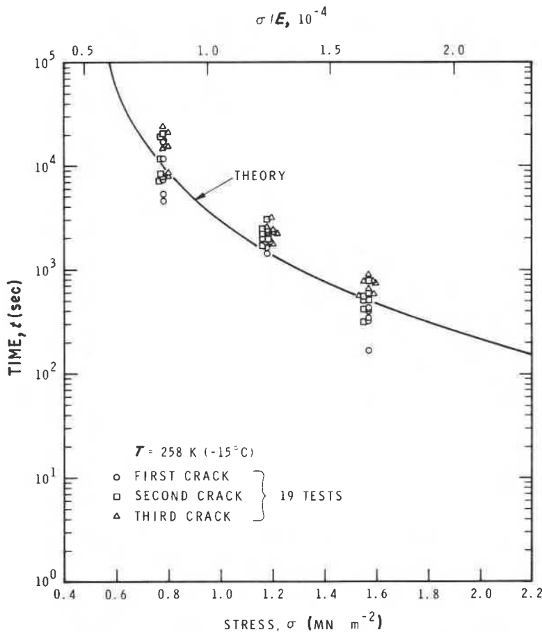
Figure 3 Dependence of time to the formation of first cracks on stress, T = 258 \text{ K} (-15^\circ \text{C}) . Experimental results are from Gold [28, 29].
