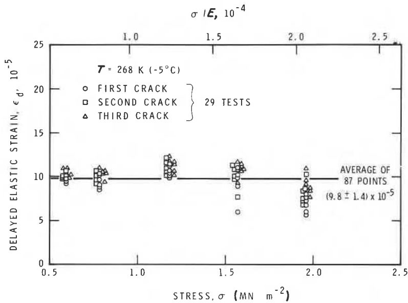
Figure 6 Computed delayed elastic strain for the formation of first three large cracks during creep in S-2 ice of average grain diameter of 4.5 mm at 268 K ( -5^{\circ}\text{C} ).
