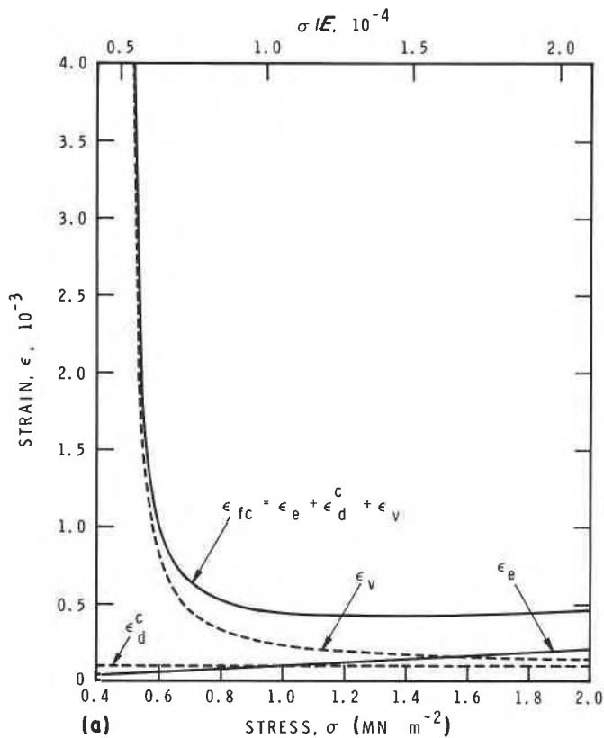
Figure 11 (a) Theoretical total strain and its three components for the formation of the first cracks at 263 K ( -10^{\circ}\text{C} ) for grain diameter of 4.5 mm. (b) Stress and temperature dependence of creep strain to the formation of the first large cracks.
