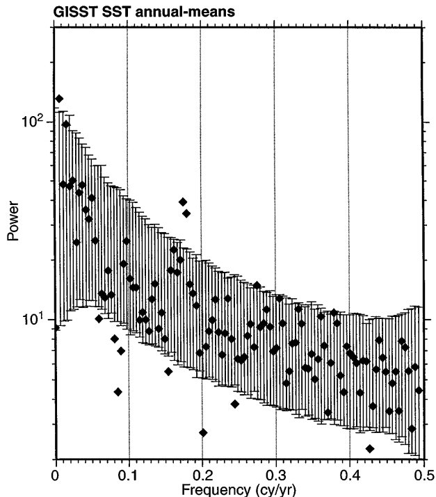
Fig. 13. Monte-Carlo significance test of North Pacific GISST annual mean SSTs. The error bars indicate the 90% confidence interval of the AR(1) noise null hypothesis. As Fig. 2
