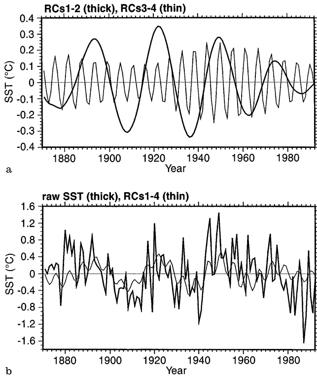
Fig. 14a, b. Indices of the leading two GISST RC pairs over the 5^\circ -box ( 35\text{--}40^\circ\text{N} , 150\text{--}155^\circ\text{W} ). a RCs 1–2 (thick line), and RCs 3–4 (thin line); b raw GISST SST (thick line), and the sum RCs 1–4 (thin line)
