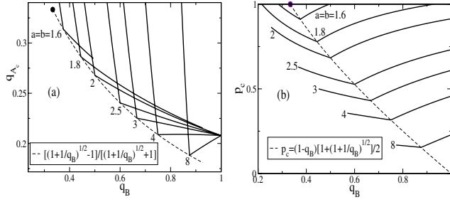
FIG. 4 (color online). The critical point parameters, q_{A_c} (a) and p_c (b), as functions of the coupling strength q_B for ER networks are plotted for different values of a = b . (a) For q_B = 1 the networks (with large degrees) have the same critical coupling strength q_{A_c} = 0.20794 . The networks with small degrees do not have first order phase transitions (no critical points for q_B ), because for large values of q_B , p_c(q_B) > 1 , which is unphysical. The range of q_B values for which the first order phase transition exists shrinks as a = b decreases and eventually disappears for a = b = 3/2 , when the critical point exists only for q_{A_c} = q_B = 1/3 and p_c = 1 . This point is marked by a solid circle.
