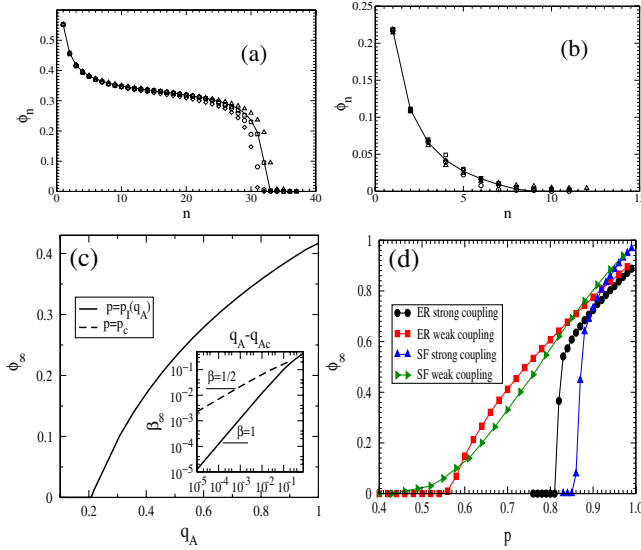
FIG. 2 (color online). \phi_\infty , the fraction of nodes in network's B giant component, after a cascade of failures in ER networks of size N_A = N_B = 8 \times 10^5 . (a) The value of \phi_n for every iteration of the first order cascades with the initial parameters p = 0.7455 , a = b = 2.5 , q_A = 0.7 , and q_B = 0.6 . (b) Similar to (a) but for the second order case with parameters p = 0.605 , a = b = 2.5 , q_A = 0.2 , and q_B = 0.75 . Symbols represent simulation results for different random realizations of the networks. Solid lines represent the solution of system (5). (c) \phi_\infty , as function of q_A computed at p = p_I(q_A) , the line of the first order phase transition, for a = 3 , b = 3 , q_B = 1 . Inset: The same results (solid line) as function of |q_A - q_{Ac}| yield a straight line with slope \beta = 1 in double logarithmic scale. If q_A is changed but p = p_c is kept constant we obtain a straight line with slope \beta = 0.5 (dashed line). (d) Simulation results for the phase transition of \phi_\infty as a function of p for ER and SF ( \lambda = 2.7 ) networks of size N = 50 K. For strong coupling between the networks we observe a jump in \phi_\infty as expected in the first order phase transition [ER (circle) and SF (up-pointing triangle)]. For weak coupling between the networks the change in \phi_\infty is gradual as expected for the second and higher order phase transitions [ER (square) and SF (right-pointing triangle)].
